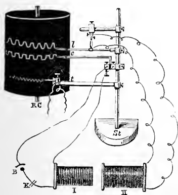
Fig. 66.—Arrangement for Estimating the Time-Relations of a Single Muscular Contraction.—B, battery; K, key in primary circuit; I., primary, II., secondary spiral, without a short-circuiting key; l , muscle lever; e , electro-magnet in primary circuit; t , electric signal; St , support; RC, revolving cylinder.
