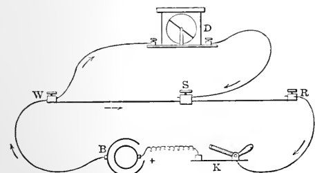
Fig. 43.—Scheme of Simple Rheocord.—B, Battery; K, key; W, R, wire; S, slider; D, detector.
