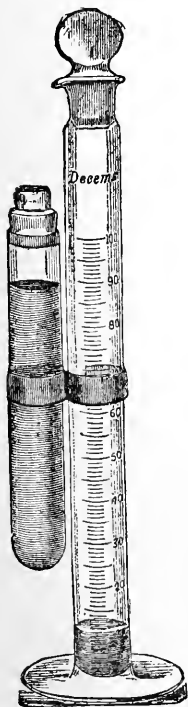
Fig. 30.—Picro-saccharimeter.
