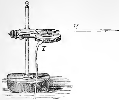
Fig. 76.—Marey's registering tambour. Metallic Capsule, T, with thin india-rubber stretched over it, and bearing an aluminium disc, which acts upon the writing-lever, H.
