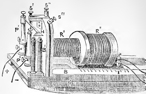
Fig. 46.—Induction apparatus of du Bois-Reymond. — R' , Primary; R'' , secondary spiral; B , board on which R'' moves; I , scale; + - , wires from battery; P, P'' , pillars; H , Neef's hammer; B' , electro-magnet; S' , binding screw touching the steel spring ( H ); S'' and S''' , binding screws to which are attached wires when Neef's hammer is not required.
