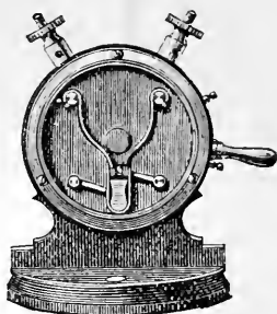
Fig 45. Thomson's Reverser.
