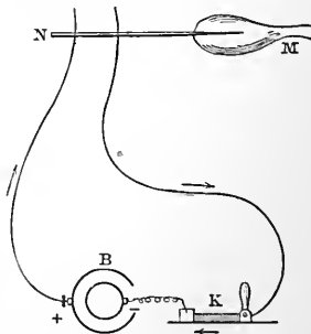
Fig. 38.—Scheme of du Bois Key.—B, battery; K, key; N, nerve; M, muscle.
