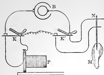
Fig. 48.—Scheme of the Break Extra-current.—B, Battery; K and K', keys; P, primary coil; N, nerve.
