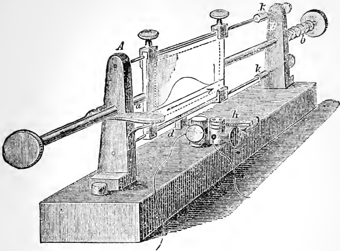
Fig. 65.—Spring Myograph.
