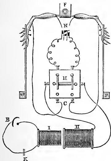
Fig. 58.—Scheme of the Curare Experiment.—B, Battery; I., primary, II., secondary spiral; N, nerves; F, clamp; NP, non-poisoned leg; P, poisoned leg; C, commutator; K, key.
