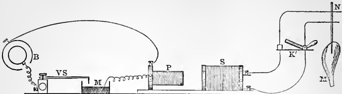
Fig. 73.—Scheme of Arrangement for Tetanus.—VS, Vibrating spring; M, cup for mercury. Other letters as before.
