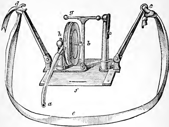
Fig. 114.—Marey's Stethograph.
