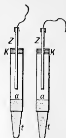
Fig. 80.—Non-polarisable Electrodes.—Z, Zincs; K, cork; a, zinc sulphate solution; t, t, clay points.
