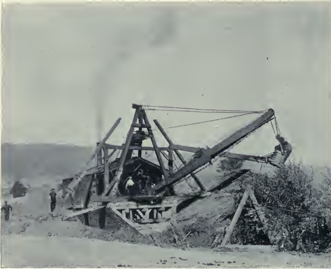
MODIFICATION OF SCOOP DREDGE FOR DITCHING.
