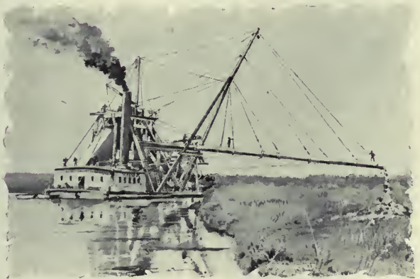
HERCULES DREDGE, "THOR."
