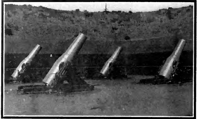
A battery of modern 12inch breech-loading mortars of our coast defense, similar to those at Corregidor.
