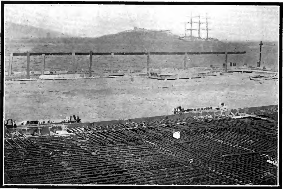
Wharf floor, showing reinforced steel construction.
