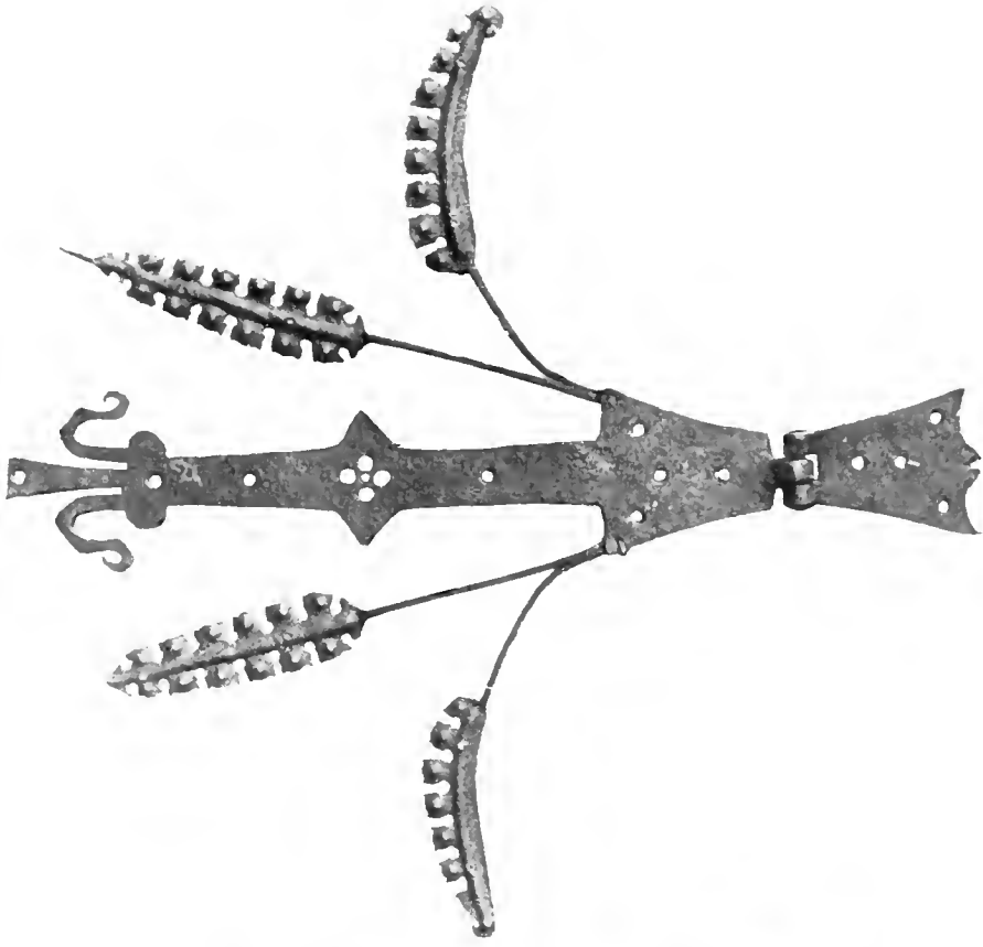
Vine-pattern hinge. French; 15th century. In the Victoria and Albert Museum, no. 670 (p. 89).
