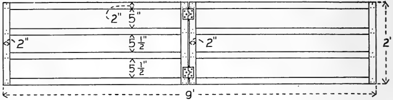
A CONVENIENT, EASILY CARRIED HURDLE.
