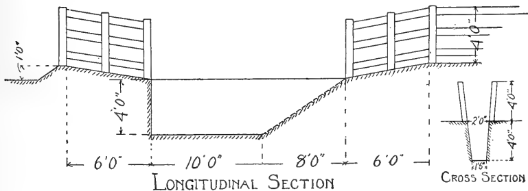
CEMENT DIPPING TANK.
