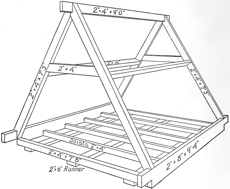
FRAME WORK OF AN "A" SHAPED PORTABLE HOG HOUSE.
