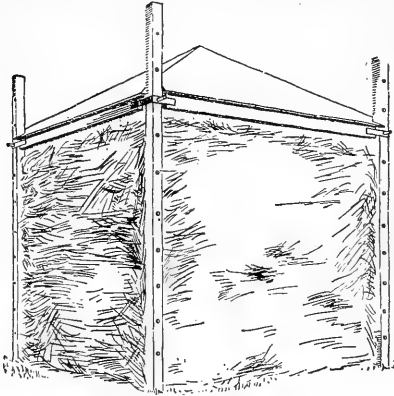
AN ADJUSTABLE ROUGHAGE STACK COVER.
