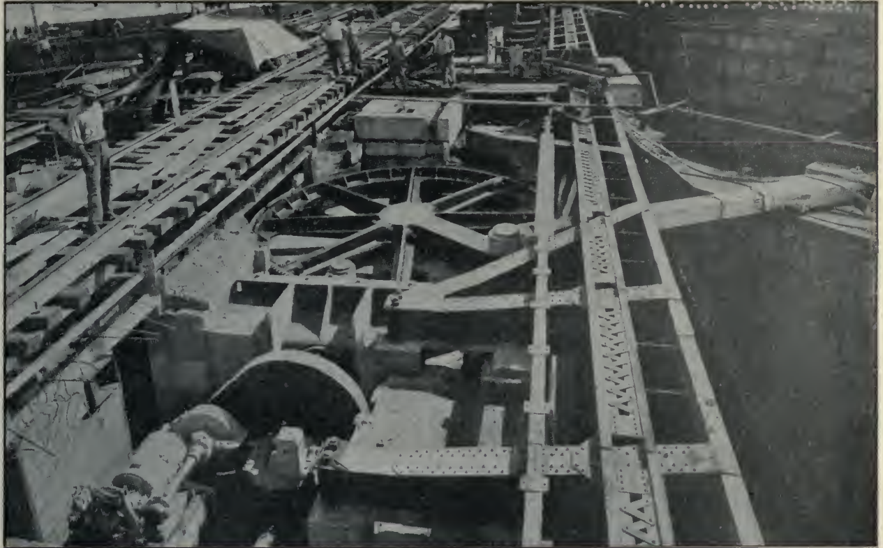
Gatun Upper Locks, Miter Gate Moving Machine, Structural Steel Girders for Towing Locomotive Track Supports in Foreground. This Photograph Was Taken in June, 1912.
