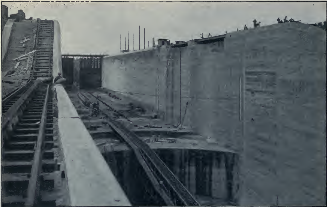
—Photo by Underwood & Underwood, N. Y. View Showing East Chamber, Lower and Middle Locks at Gatun, with Section of Rack Track on East Wall. Photographed March 14, 1912.
