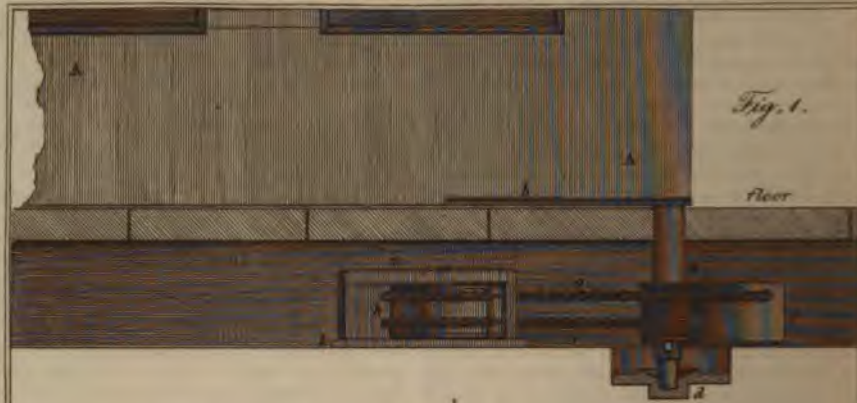
Mr. Morris's Swing Door Hinge.
