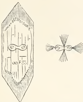
FIG. 3.—Olivine crystal seen parallel to \infty P\tilde{\infty} and showing excellent cleavage along \infty P\tilde{\infty} , and poorer cleavage along OP . The fibrous bastitic mineral into which it is altered has fibres parallel to the principal cleavage. A bisectrix occurs at right angles to the section, and the plane of the optic axis is parallel to the base
