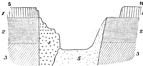
FIG. 2.—De Beers Mine, 1885. (Sketch by Professor Lewis from the Colonial Exhibition, 1886.) 1, lensalt; 2, shale; 3, hard ground; 4, floating reef (true eruptive rock, with more bronzite, no enclosures, no diamonds); 5, diamond-bearing rock
