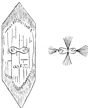
FIG. 3.—Olivine crystal seen parallel to \infty P\bar{\infty} and showing excellent cleavage along \infty P\bar{\infty} , and poorer cleavage along OP . The fibrous bastitic mineral into which it is altered has fibres parallel to the principal cleavage. A bisectrix occurs at right angles to the section, and the plane of the optic axis is parallel to the base
