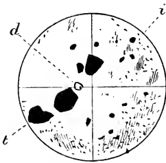
FIG. 23.—Microscopic section of the Kimberley peridotite. i , ilmenite; t , titanite; d , diamond (?)
