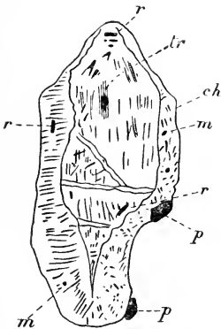
FIG. 6.—Diagrammatic. r , rutile needles; tr , tremolite; ch , chrysothile; m , magnetite or chromite; p , perovskite
