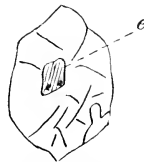
FIG. 18.— e , enstatite, with specks of biotite
