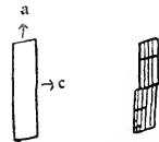
FIG. 31.—Cyanite? a, lavender; c, greenish
