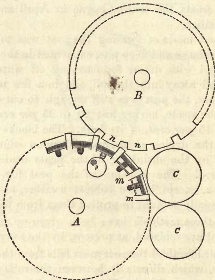
Fig. 11 —WEBER'S PEAT MOULDING MACHINE.
