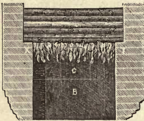
Fig. 24.—WEBER'S CHARRING FURNACE.—TRANSVERSE SECTION.
