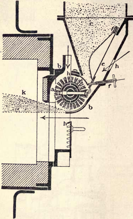
FIG. 192—Schwartzkopf's Powder-firing Apparatus.
