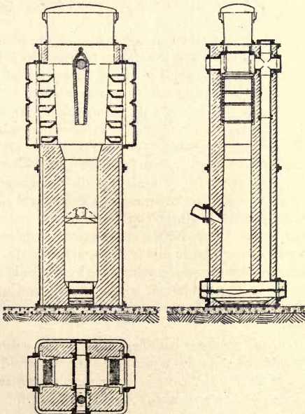
FIG. 204—Körting's Peat Gas-producer.
