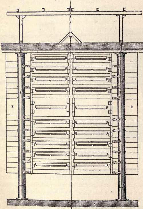
FIG. 146—Steam plate Drier (side view)
