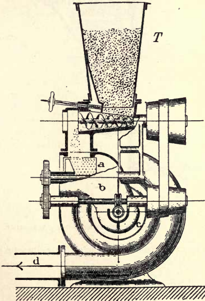
FIG. 191—F. de Camp's Powder-firing Apparatus.
