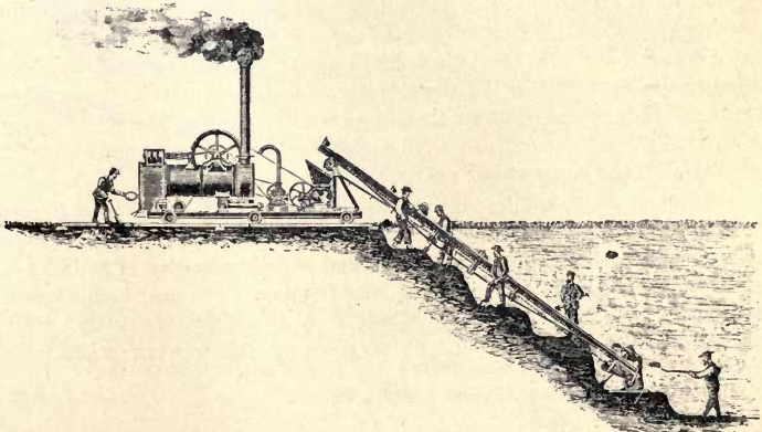
FIG. 69—R. Dolberg's Peat Plant with end elevator.
