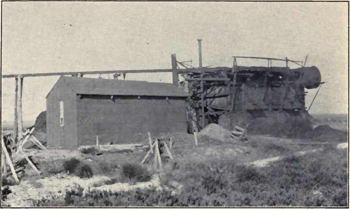
Peat Plant at Moselund, Denmark.
