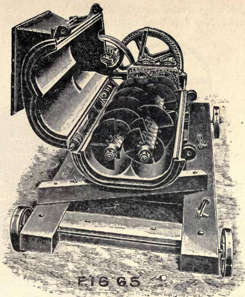
FIG. 65—R. Dolberg's Peat Machine No. 1b (interior).
