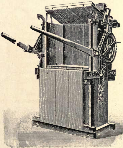
FIG. 224—Moss Litter Press for Hand-power.
