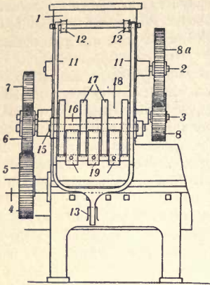
Schlickeysen's Peat Machine No. 3.
