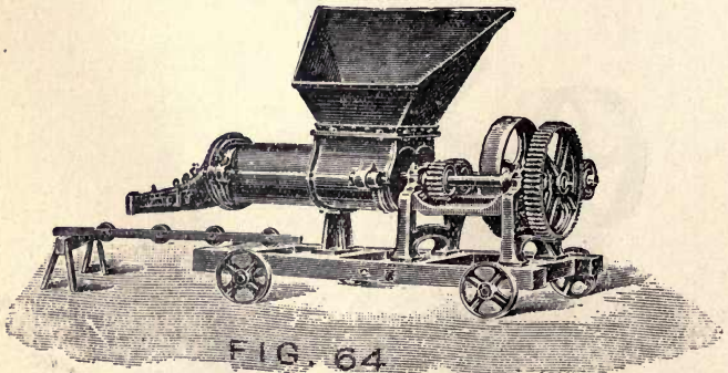
FIG. 64—R. Dolberg's Peat Machine No. 1b (exterior).
