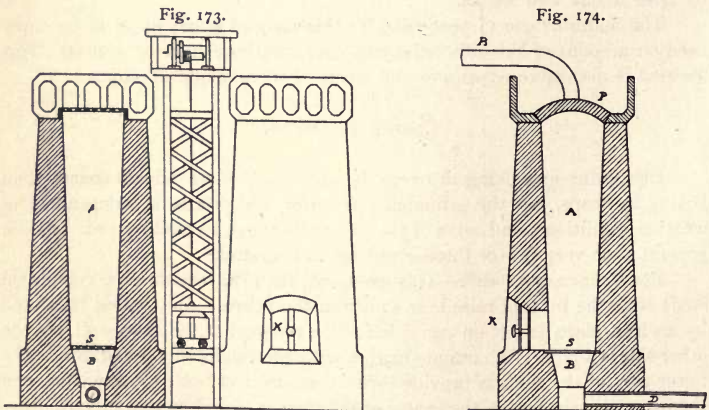
The Wagenmann Peat Coking Oven.
