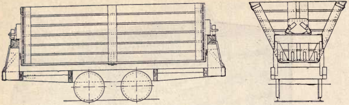
FIG. 127—Car for transport of dried Peat.
