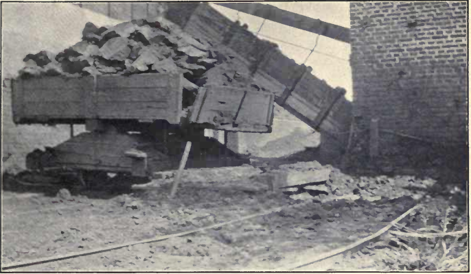
Car for Transport of Raw Peat, Ökaer, Denmark.
