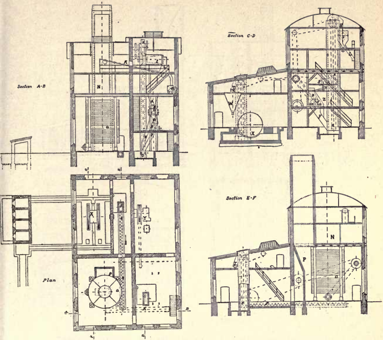
FIG. 162—Peat Briquetting Plant with One Press and Steamplate Drier.
