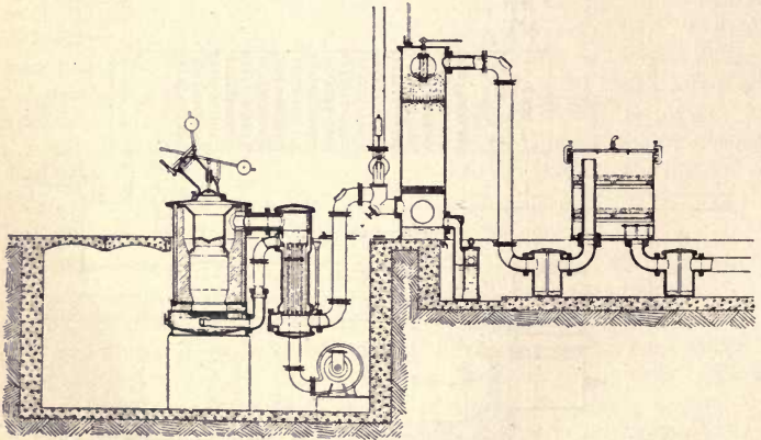
FIG. 202—Körting Gas-producer Plant for Anthracite or Coke.
