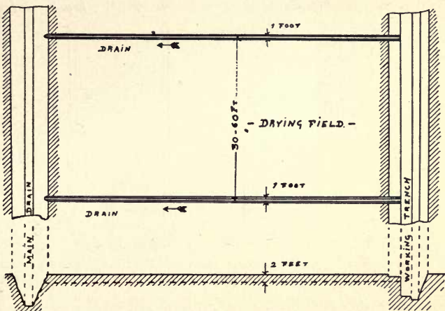
FIG. 2—Method of Drainage.
