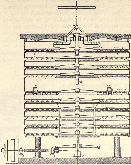
FIG. 147—Steam plate Drier (section).
