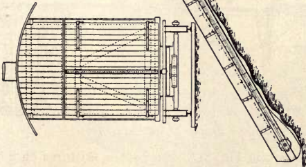
Peat Plant with Anrep-Svedala Peat Machine.
