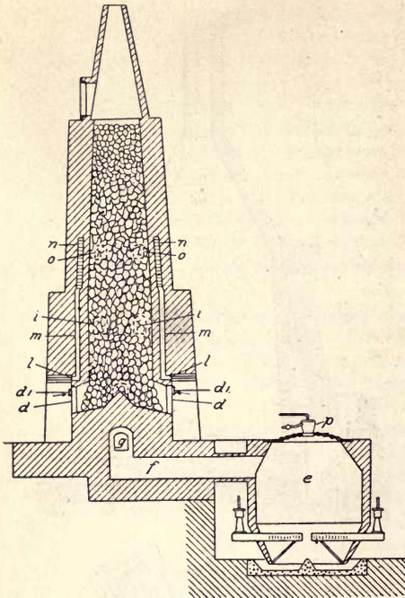
FIG. 198—Lime Kiln Fired with Producer-gas.
