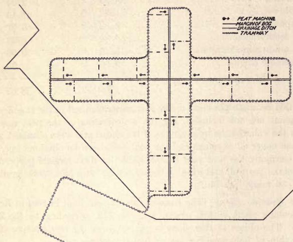
FIG. 180—Peat Bog at Redkino, Russia.
