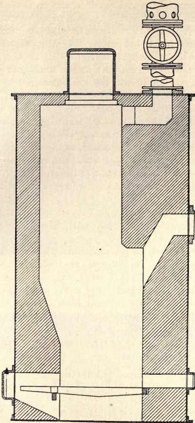
FIG. 203—Körting's Lignite Briquette Gas-producer.
