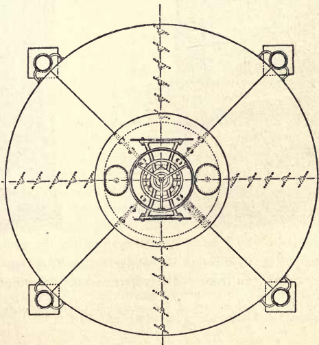
FIG. 148—Steam plate Drier (plan).
