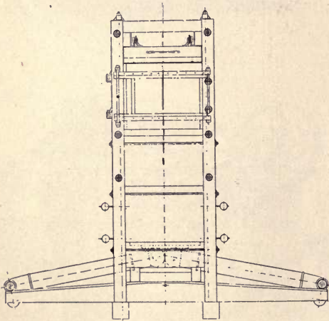
FIG. 226—Moss Litter Press for Motor-power.
