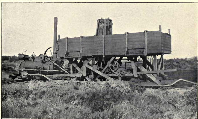
Peat Plant at Herning, Denmark.
