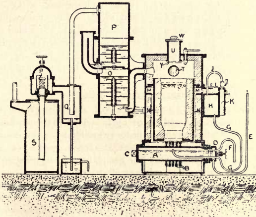
FIG. 200—Bénier Gas-producer Plant for Anthracite or Coke.
