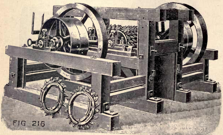
FIG. 216—A. Heinen's Moss Litter Disintegrator for Motor-power.
