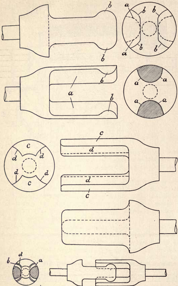
FIG. 120—Coupling to A. Körner's Peat Conveyor.
