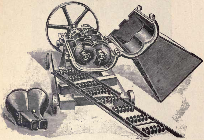
FIG. 67—R. Dolberg's Peat Machine No. 1c (interior).
