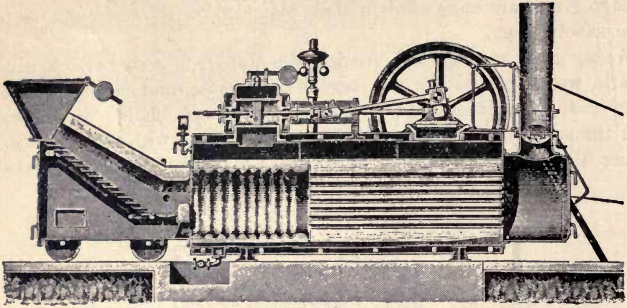
FIG. 185—Locomobile with Step-grate, from H. Lanz, Mannheim, Germany.
