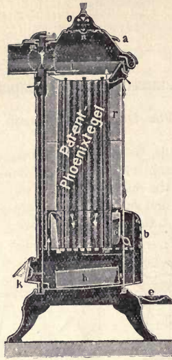
FIG. 183—Ankarsum's Peat Stove.
