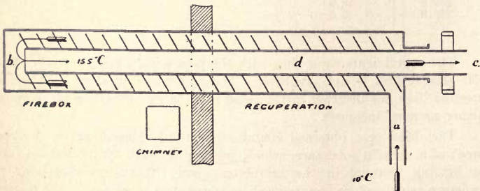
FIG. 171—Theoretical working of a Wet Carbonizing Oven.
