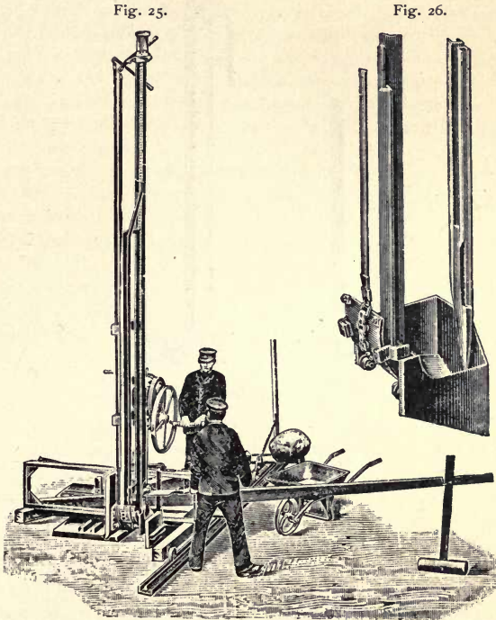
R. Dolberg's Cutting Machine.
