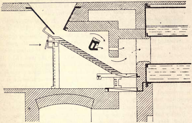
FIG. 189—Keilmann & Völcker's Half-gas Furnace.
