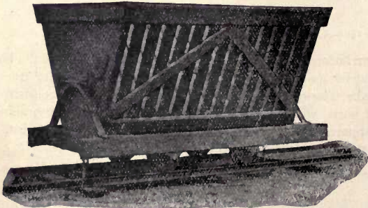
FIG. 123—Car for transport of dried Peat.
