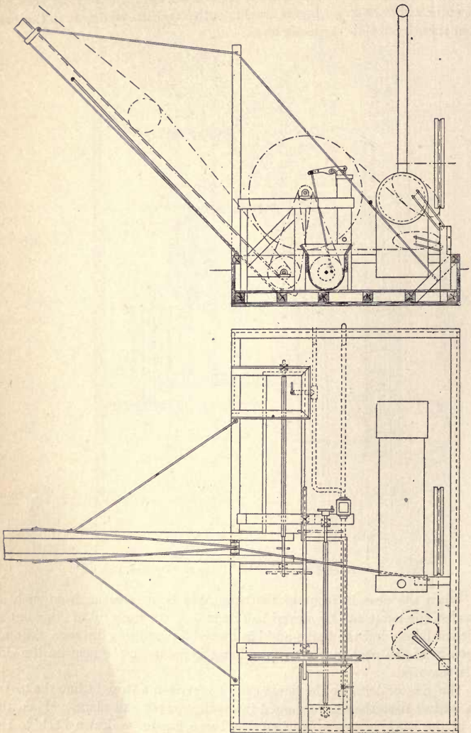
FIG. 44—Floating Peat Plant at Aamosen, Denmark.
