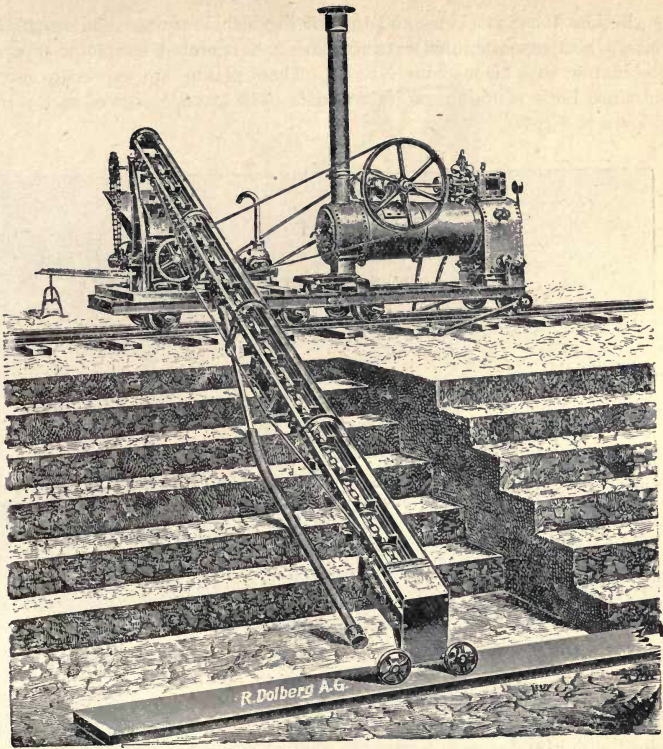
FIG. 68—R. Dolberg's Peat Plant with side elevator.
