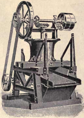
FIG. 220—A. Heinen's Peat Mull Mill.
