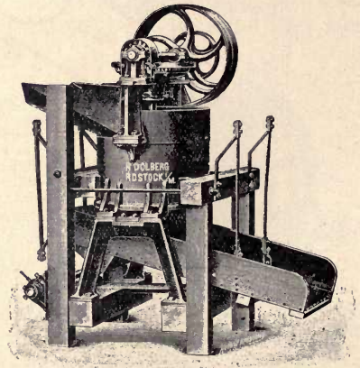
R. Dolberg's Peat Mull Mills.
