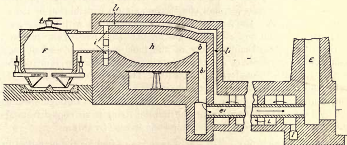
FIG. 196—Reverberatory Furnace, Fired with Producer-gas.
