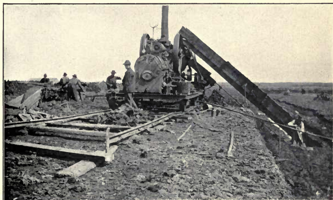
Peat Machine at Triangel, Germany.
