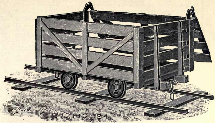
FIG. 124—Car for transport of dried Peat.
