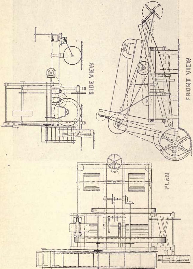
FIG. 167—The Dobson Peat Excavator.
