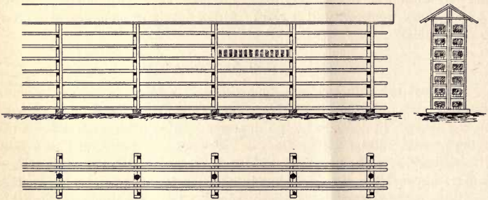
FIG. 29—Drying Shed.
