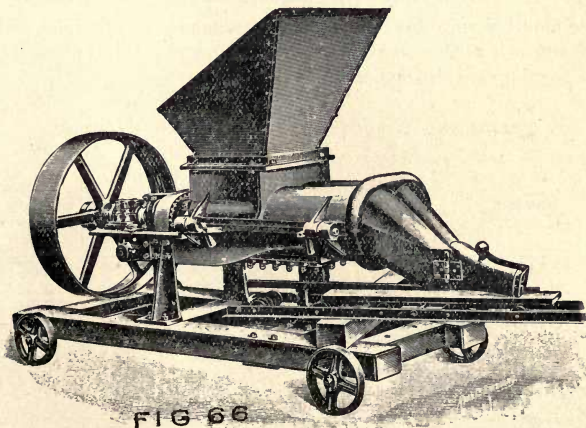
FIG. 66—R. Dolberg's Peat Machine No. 1c (exterior).
