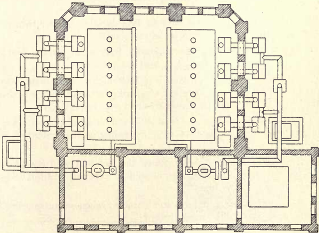
FIG. 179—8-Oven Peat Coking Plant at Redkino, Russia.
