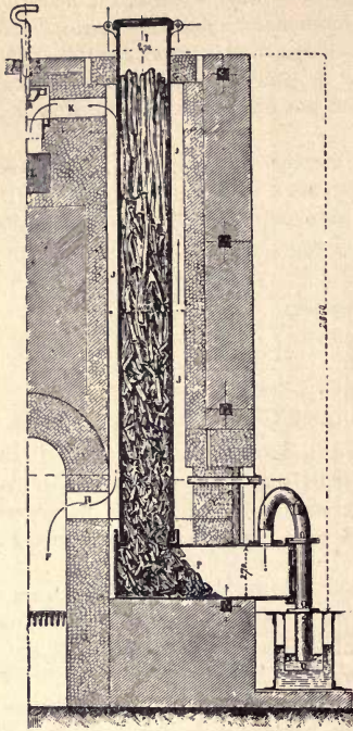
FIG. 211—Riché Gas-producer.
