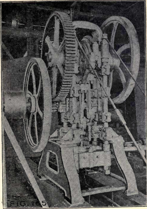
FIG. 165—The Dickson Peat Briquetting Press.
