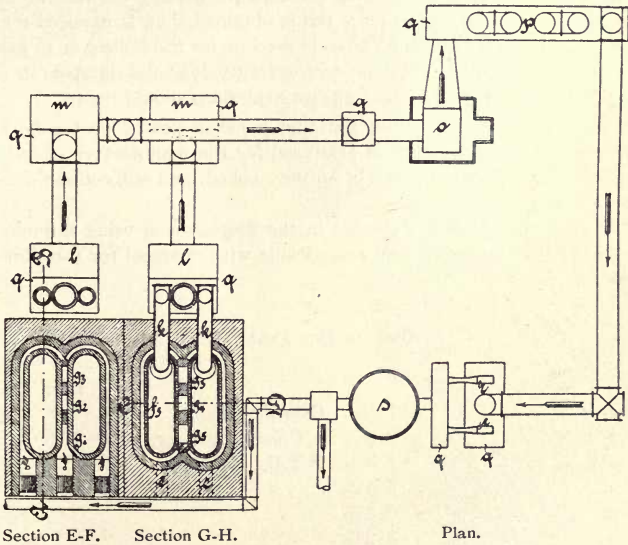
M. Ziegler's Peat Coking Retorts.
