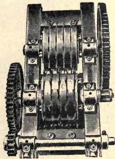
R. Dolberg's Moss Litter Disintegrator for Hand-power.
