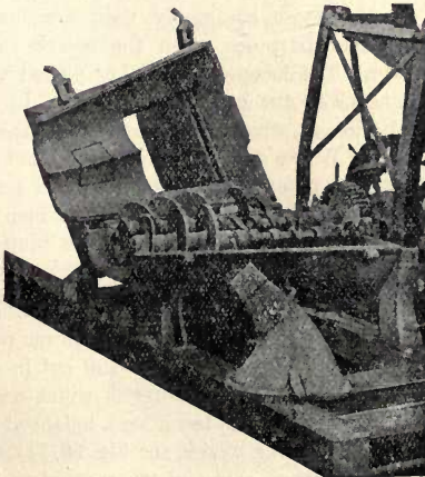
FIG. 91—Akerman's Peat Machine.
