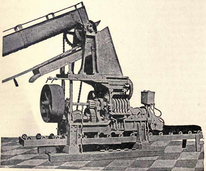
FIG. 55—Schlickeysen's Peat Machine No. 3.
