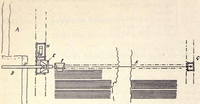
FIG. 45—Peat Plant at West Torup, Sweden.
