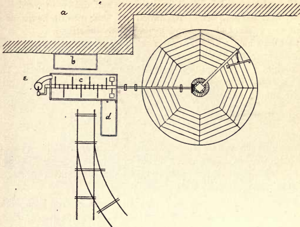
FIG. 32—General arrangements at a small Peat Plant.
