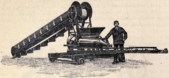
FIG. 92—Åkerman's Peat Machine.
