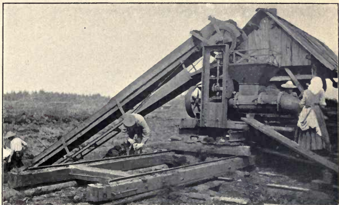
Peat Machine at Feilenbach, Germany.
