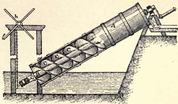
FIG. 1—Closed Water-screw.
