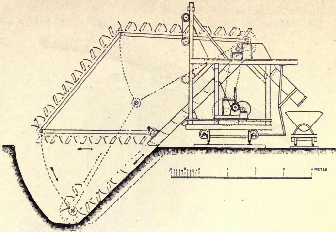
FIG. 58—Schlickeyesen's Peat Excavator.
