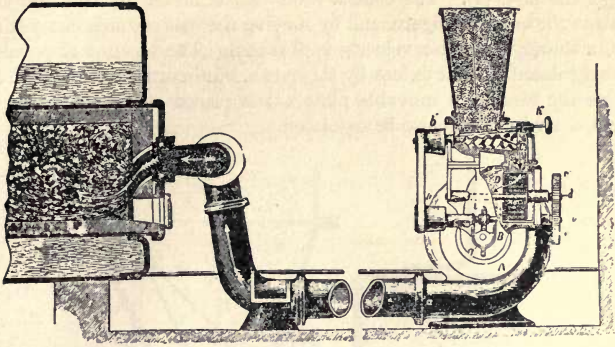
FIG. 190—F. de Camp's Powder-firing Apparatus.
