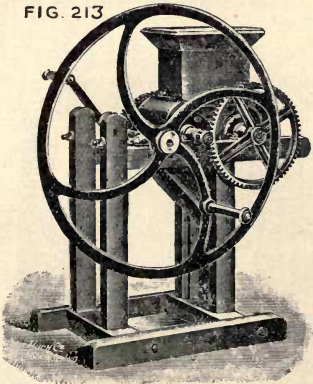
R. Dolberg's Moss Litter Disintegrator for Hand-power.
