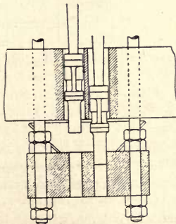
FIG. 166—Die Block to the Dickson Peat Press.
