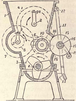
Schlickeysen's Peat Machine No. 3.
