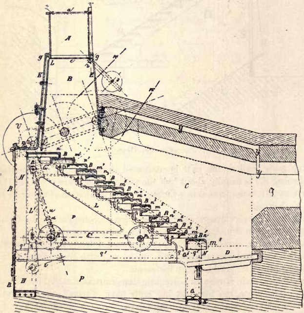
FIG. 186—Kowalsky's Step-grate.
