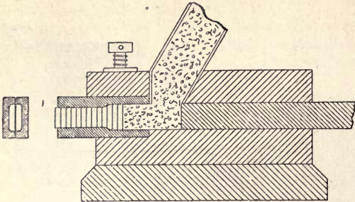
FIG. 155—Section of Briquette Press.
