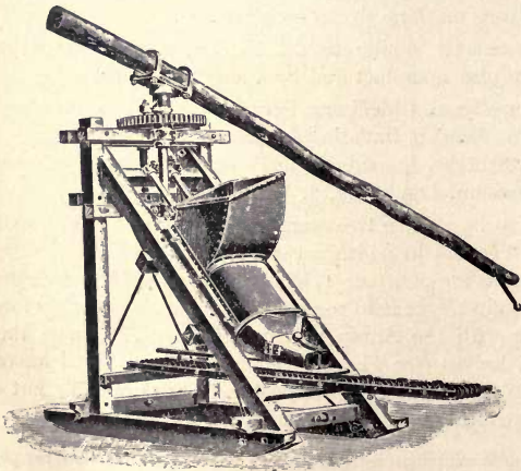
FIG. 60—R. Dolberg's Peat Machine No. 2 (exterior).
