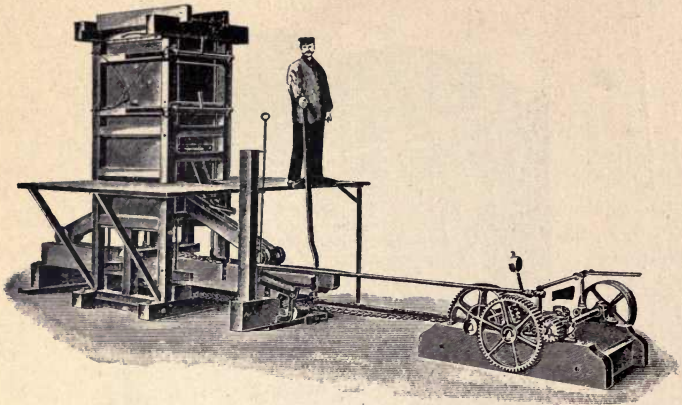
FIG. 225—Moss Litter Press for Motor-power.
