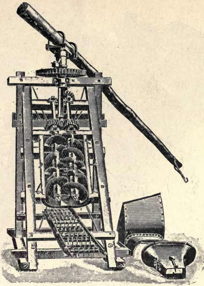
FIG. 61—R. Dolberg's Peat Machine No. 2 (interior).
