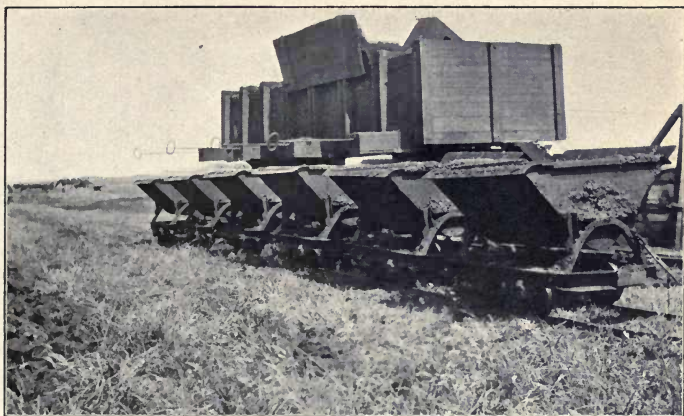
Bin and Peat Cars at Aamosen, Denmark.
