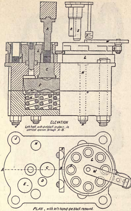
FIG. 170—Die Block and Bed to the Dobson Press.
