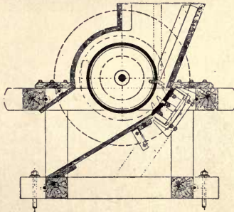
FIG. 219—Abjörn Anderson's Moss Litter Disintegrator for Motor-power.
