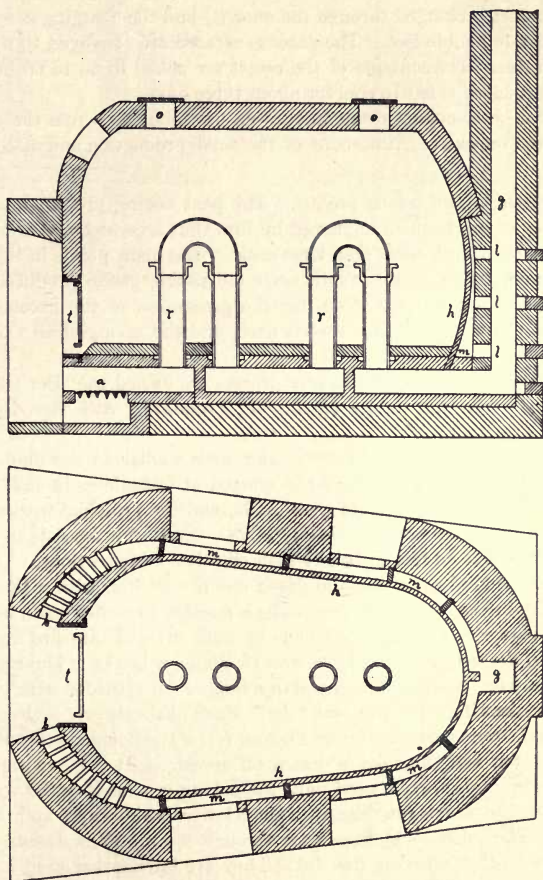
FIG. 175—The Lottmann Peat Coking Oven.
