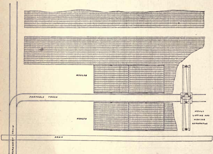
FIG. 40—Drying Field at Herning, Denmark.
