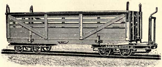
FIG. 126—Car for transport of dried Peat.
