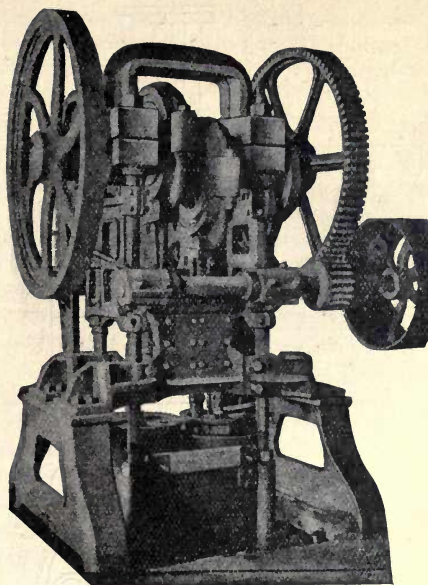
FIG. 169—The Dobson Peat Briquetting Press.
