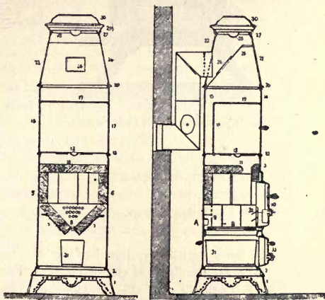
FIG. 182—Rech's Peat Stove.
