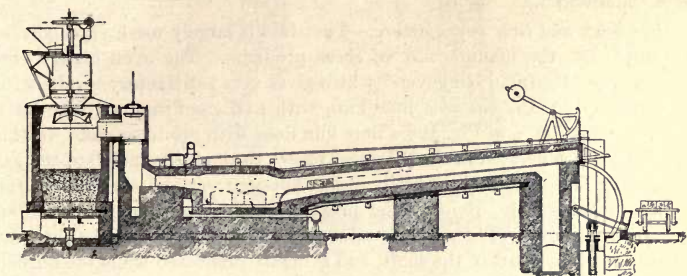
FIG. 195—Bildt's Producer combined with Re-heating Furnace.
