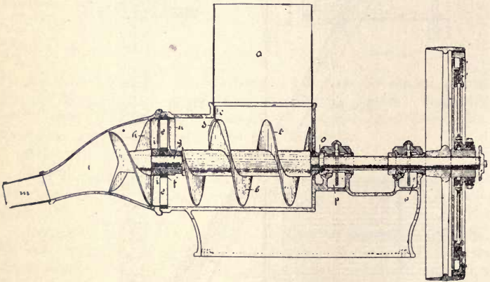
FIG. 88—Svedala Peat Machine No. 2.
