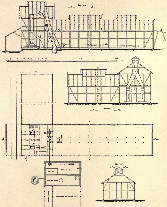
FIG. 228—Moss Litter Plant with Two Presses.
