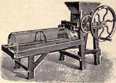
FIG. 215—A. Heinen's Moss Litter Disintegrator for Hand-power.
