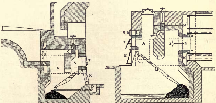
C. Reich's Half-gas Furnace.
