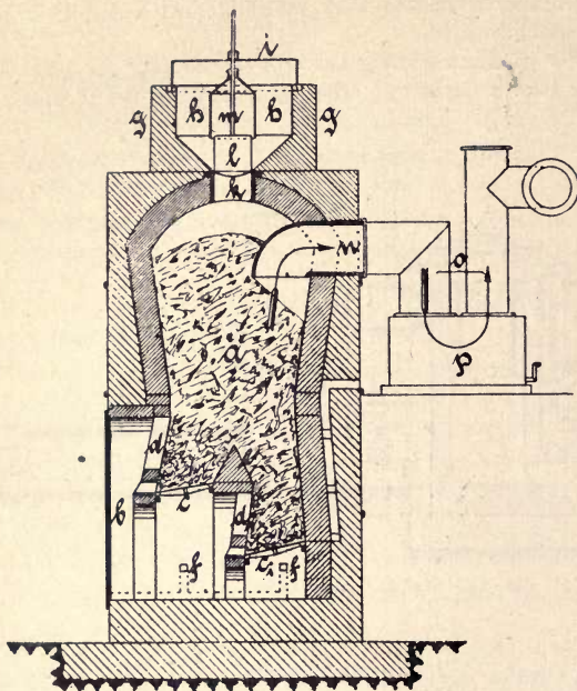
FIG. 210—M. Ziegler's Peat Gas-producer.
