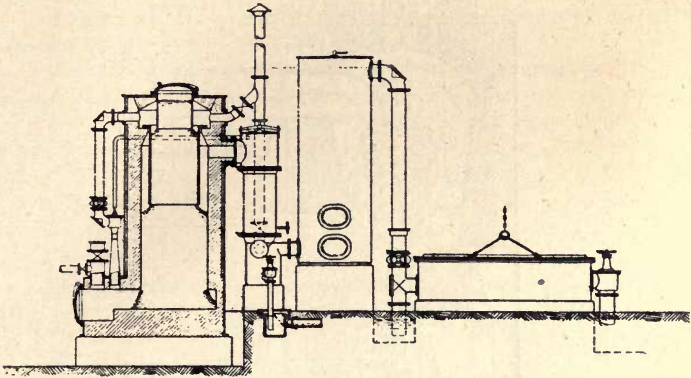
FIG. 209—Pintsch Gas-producer for Bituminous Fuels.
