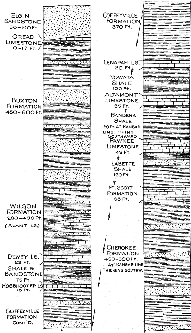
Fig. 16.—Columnar section of the Pennsylvanian rocks in northeastern Oklahoma.
