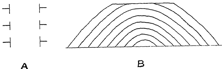
Fig. 11.—A. Map record of dip and strike showing anticlinal structure. B. The structure of the area shown in A in cross section. (Chamberlin and Salisbury.)
