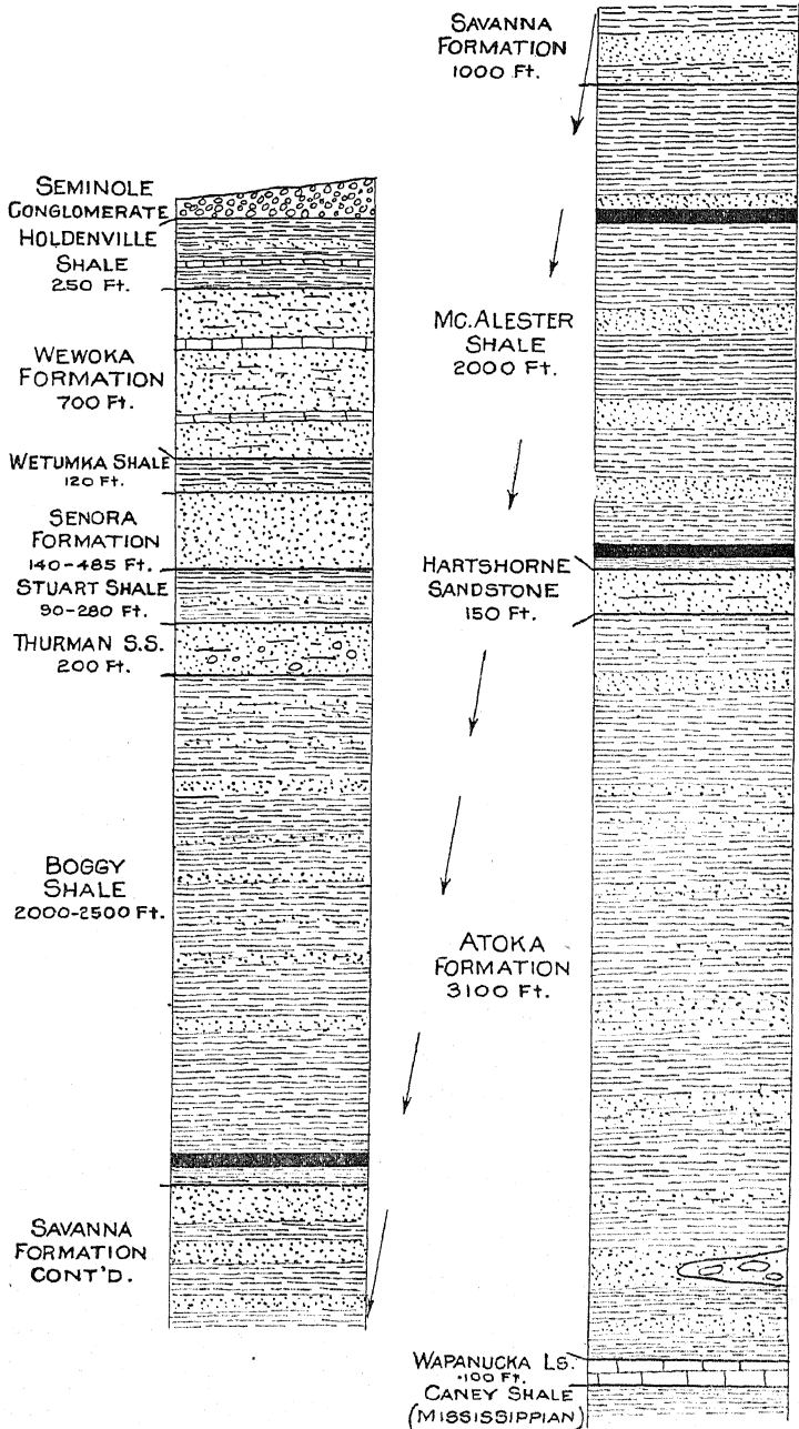
Fig. 17.—Columnar section of the Pennsylvanian rocks in the region south of Arkansas River.
