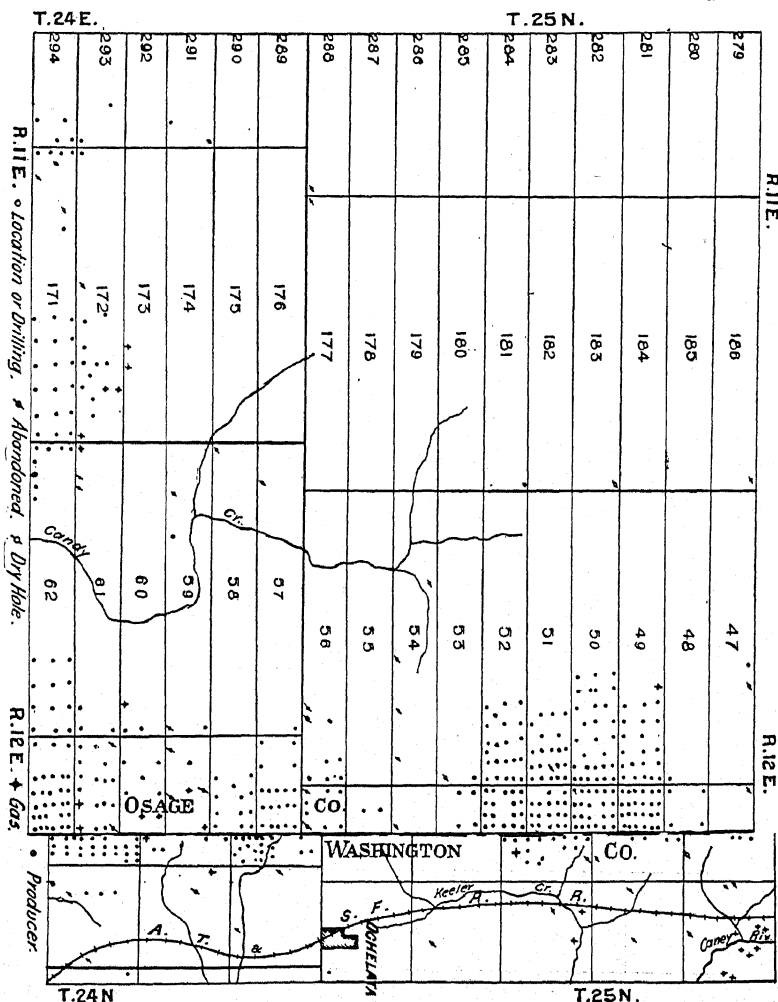
Fig. 34.—Development of north part of the Avant-Ochelata pool.
