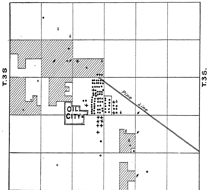
Fig. 37.—Development of the Wheeler pool.
