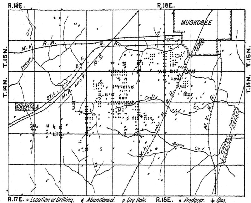
Fig. 33.—Development of the Muskogee pool.
