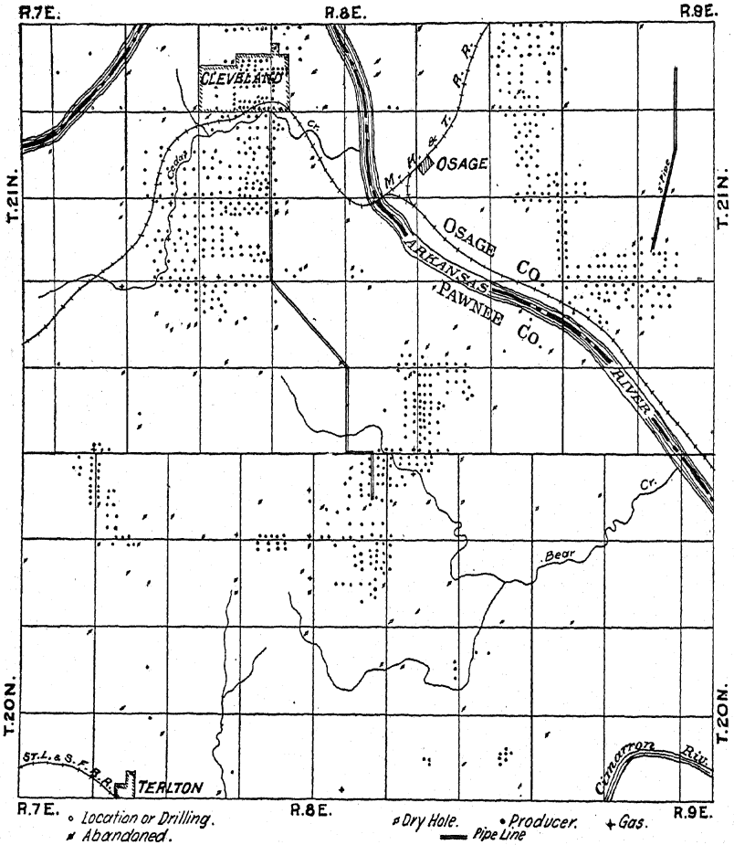
Fig. 36.—Development of the Cleveland and Osage Junction pools.
