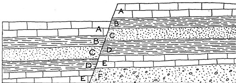
Fig. 6.—Diagram of fault.
