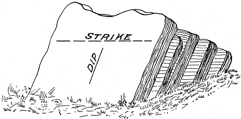
Fig. 4.—Diagram illustrating dip and strike.
