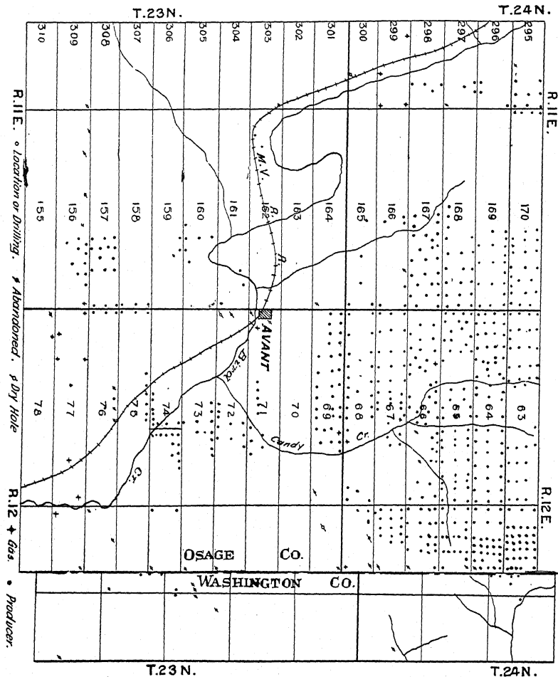
Fig. 35.—Development of south part of the Avant-Ochelata pool.
