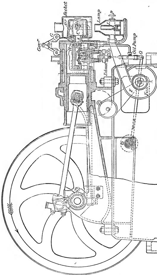
FIG. 353.—HORNSBY-AKROYD OIL-ENGINE.
