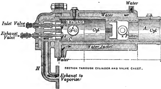
FIG. 350.—PRIESTMAN OIL-ENGINE.
