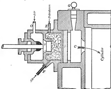
FIG. 348.—BRAYTON OIL-ENGINE.
