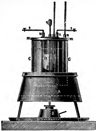
FIG. 230.—ENGLER'S ELECTRIC TESTER.
