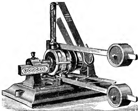
FIG. 277.—INGRAM-STAFFIER TESTER.
