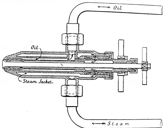
FIG. 331.—RUSDEN-EELES BURNER.
