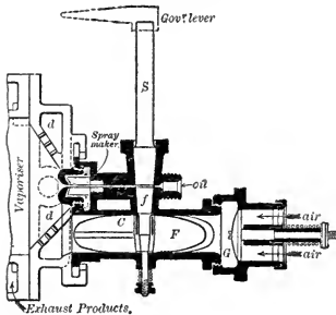
FIG. 351.—PRIESTMAN SPRAY-MAKER.
