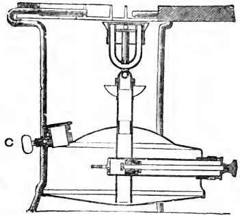
FIG. 309.—SECTION OF THE ROARER PRIMUS STOVE.
