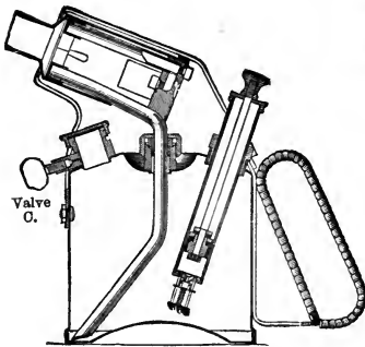
FIG. 308.—SECTION OF "AETNA" BLOW-LAMP.
