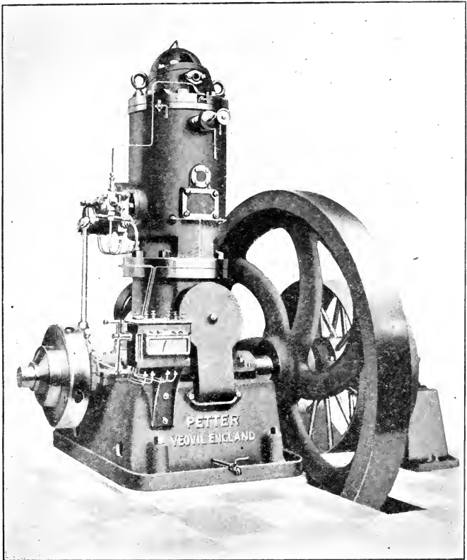
FIG. 355.—SINGLE-CYLINDER TWO-STROKE CYCLE HEAVY-OIL ENGINE BY MESSRS. PETTER, LTD., YEovil.
