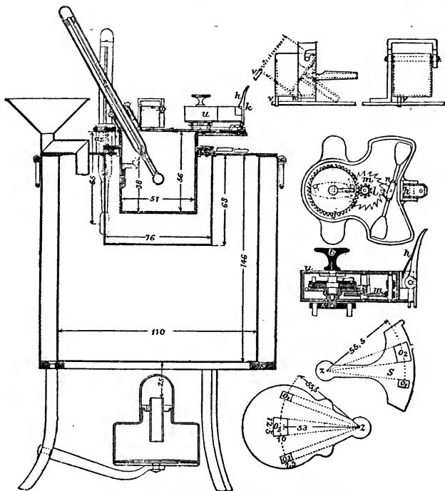
FIG. 227.—ABEL-PENSKY TESTING INSTRUMENT.
