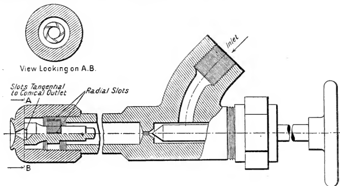
FIG. 342.—GORDEJEFF BURNER.
