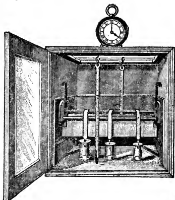
FIG. 218.—REDWOOD WICK-TESTER.
