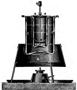
FIG. 230.—ENGLER'S ELECTRIC TESTER.
