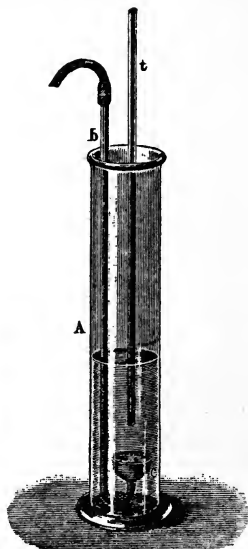
FIG. 238.— BEILSTEIN TESTER.
