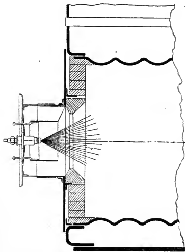
FIG. 344.—WALLSEND-HOWDEN SYSTEM FOR NATURAL DRAUGHT.
