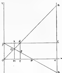
Ox = ax = A Oy = cx = C bx + cx = B The equation for the curve O G P is Bx^2 + Axy - ACx + ACy - Bxy - Ay^2 = 0 FIG. 1
