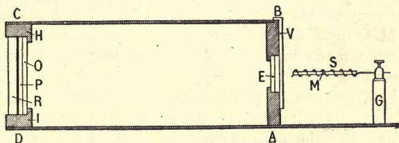
FIG. 19.—Autochrome Copying Camera.
