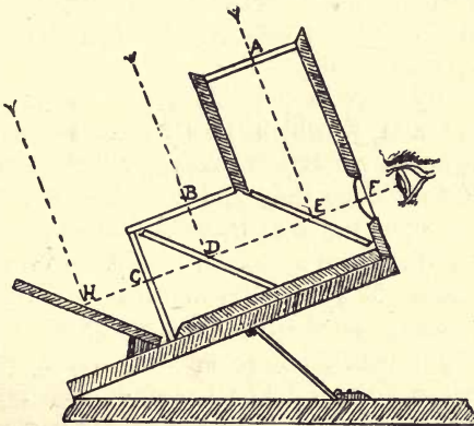
FIG. 21.—Ives' Kromskop, showing how the pictures are combined.
