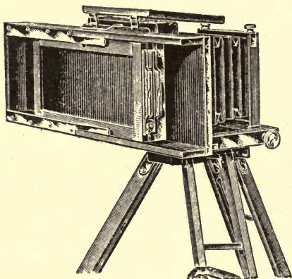
FIG. 22.—Sanger-Shepherd's Three-colour Plate Camera.
