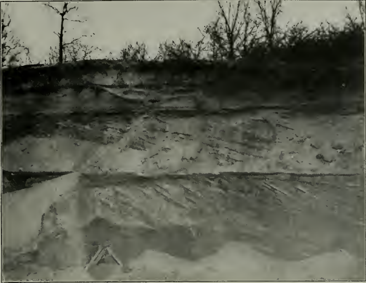
A. Stratified drift at Overholser's pit, Joliet.
