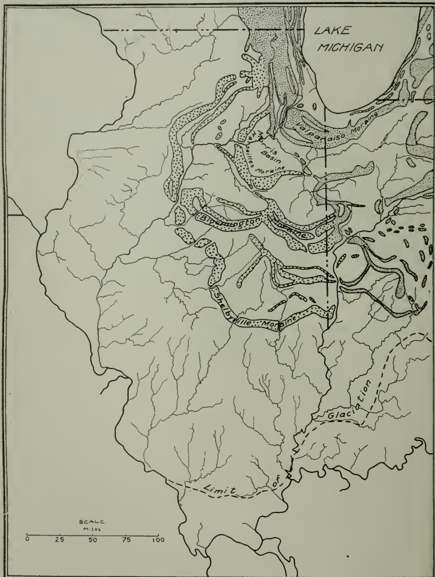
FIG. 6. Moraines and other limit of drift in Illinois. After Leverett, U. S. Geol. Surv.)
