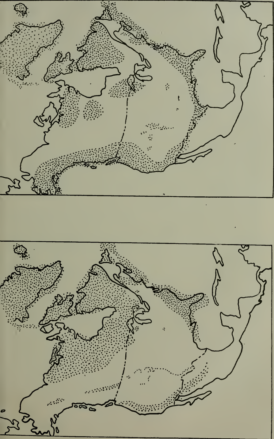
FIG. 3. North America during (a) Potsdam, or later Cambrian, and (b) Trenton, or middle Ordovician time. The unshaded areas were probably wholly submerged, the shaded areas were probably land.
