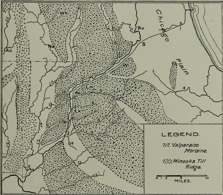
FIG. 10. Map of the lower Des Plaines river, showing towns, tributaries, and distribution of drift. Rv, Riverside; S, Summit; Wl, Willow Springs; Lm, Lemont; Ro, Romeo; Lk, Lockport; J, Joliet; N. L., New Lenox; C, Channahon; Wh, Wheaton; Na, Naperville; Au, Aurora; 1, Salt creek; 2, Chicago river; 3, Flag creek; 4, Calumet river; 5, Long run; 7, Fraction run; 8, Spring creek; 9, Hickory creek; 10, Sugar creek; 11, Jackson creek; 12, Prairie creek; 13, Rock creek; 14, Dupage river; 15, Ausable creek; 16, Fox river; 17, Buffalo creek; 18, Isle la Cache creek; 19, Mink creek; 20, Crystal run. Drift plotted from U. S. Geol. Surv., Monog. 38, by Leverett, with minor changes.
