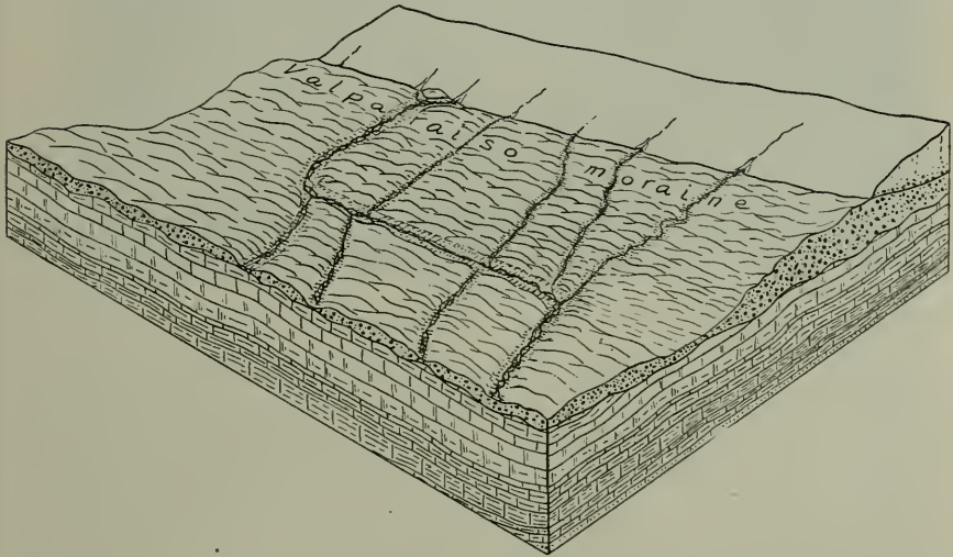
FIG. 9. A later stage than that of Fig. 8. The ice border has receded to the east side of the Valparaiso moraine. Aggrading rivers from it pass down the valleys of Hickory creek, Spring creek, Fraction run, Long run, the "Sag," and the Des Plaines valley. Distributaries occupy the transverse passages in the outer ridge, in the foreground.
