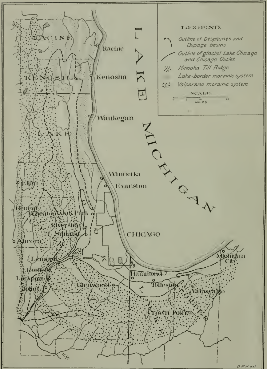
FIG. 1. Map of the Des Plaines basin and vicinity. The distribution of glacial drift is taken from Leverett's map in Monograph 38, U. S. Geol. Surv. (in Illinois), and from Alden's map in Prof. Paper 34, U. S. Geol. Surv. (in Wisconsin).
