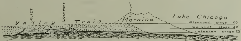
FIG. 12. Diagram showing how the removal of a sill of bed rock in the Chicago outlet, by "stoping," may have caused the sudden drop in level of the lake from the Calumet to the Toleston.
