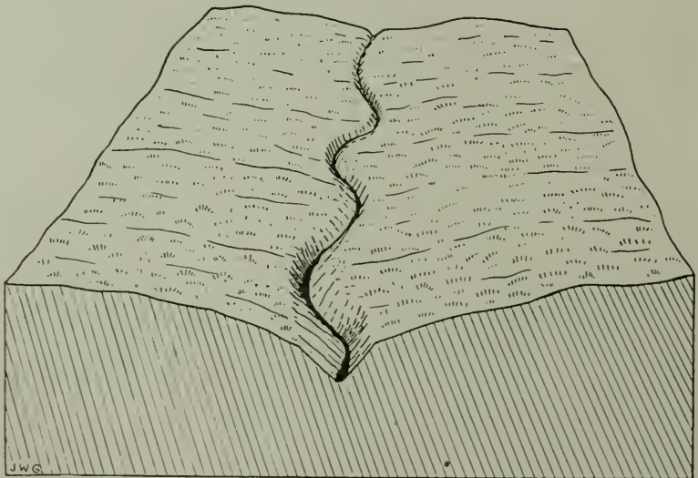
FIG. 14. A crooked gully in an early stage of development.
