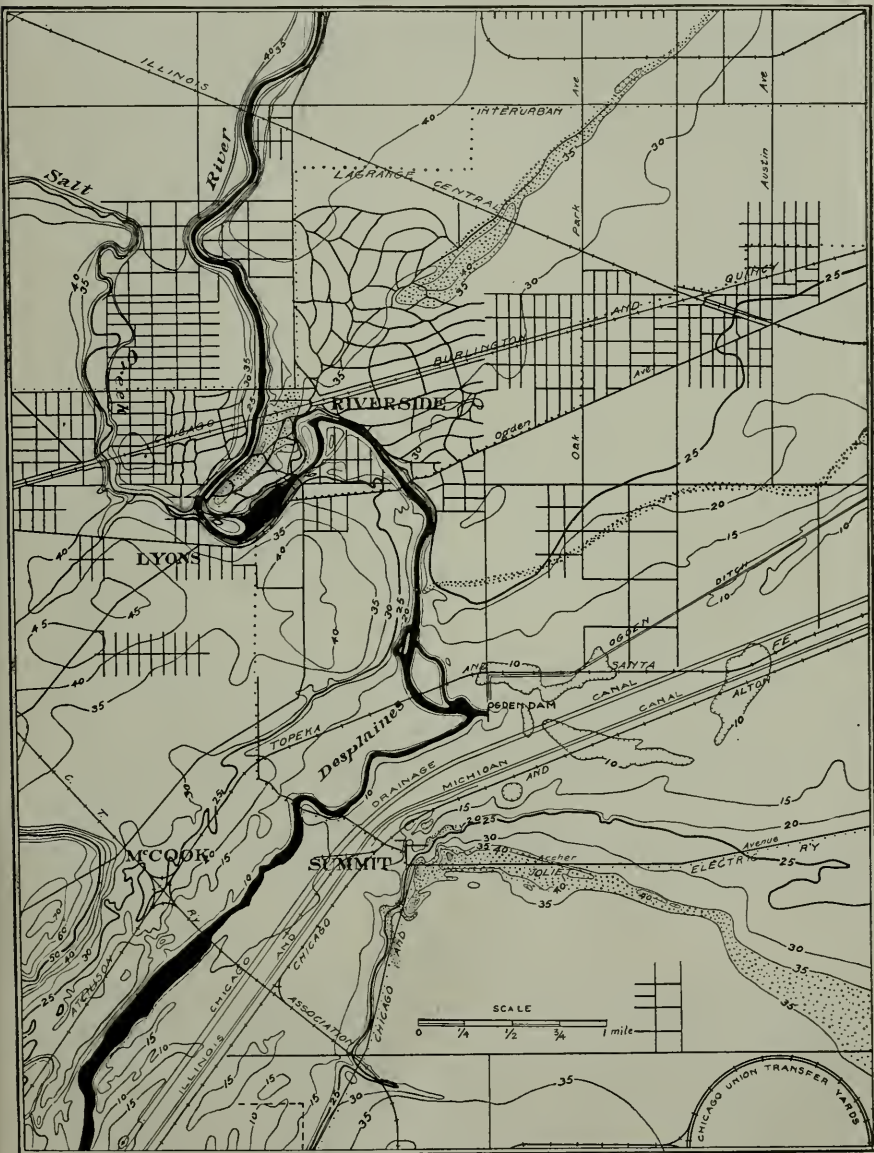
FIG. 19. Map of the district about Riverside and Summit (from map of the Sanitary district). Contour interval, 5 feet above Chicago datum. Beach ridges indicated by dotted pattern.
