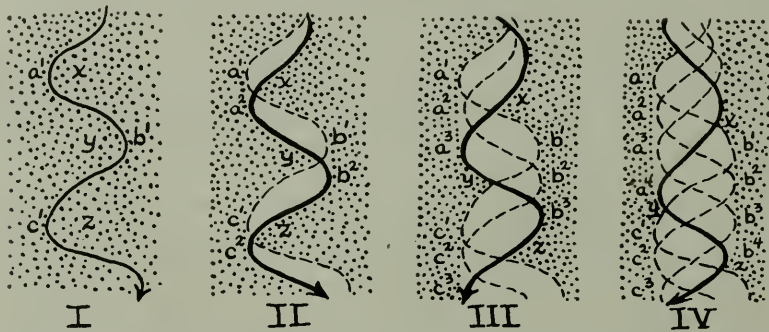
FIG. 21. Diagrams showing the development of a straight walled, flat floored valley, by the trimming away of spurs as the bends of the stream migrate down-valley. The river is flowing in the direction of the arrow. Four stages are shown. In I a_1 , b_1 , c_1 are three bends, which lie between three alternating spurs, x , y , z . The valley bottom is narrow—no wider than the stream. In II the tendency of the stream to cut on the down-valley side of each bend has shifted a_1 , b_1 , and c_1 to the positions a_2 , b_2 , c_2 , leaving stretches of straight valley walls, a_1 - a_2 , b_1 - b_2 , c_1 - c_2 . Across the river at each bend a portion of the up-valley side of each spur, x , y , z , has been trimmed away, sharpening these spurs. A flat floor, of variable width (un-shaded) has thus been produced. In III the process has continued. The bends have migrated down-valley to a_3 , b_3 , c_3 . The stretches of straight valley wall have been lengthened, a_1 - a_3 , b_1 - b_3 , c_1 - c_3 . The spurs x , y , z , have been half consumed by the trimming away of their up-valley sides. The valley floor has been much widened. In IV a still later stage has been reached. The bend a has shifted down-valley nearly to the position c , extending the straight wall a_1 - a_4 nearly far enough to consume the spur y . This spur is now very blunt, and will be wholly consumed by the time bend a has migrated down-valley to the very position which the next bend below it, c , originally had. The other spurs, x and z , have been similarly blunted, and will soon be consumed. The valley will then be straight sided, flat floored, and as broad as the swing of the bends, i. e., as the meander belt of the river.
