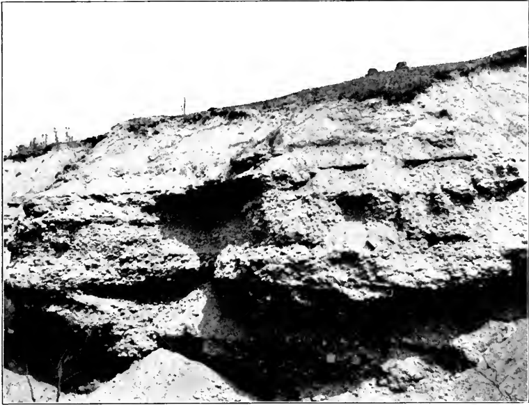
B. Exposure of Joliet conglomerate near Spring creek.
