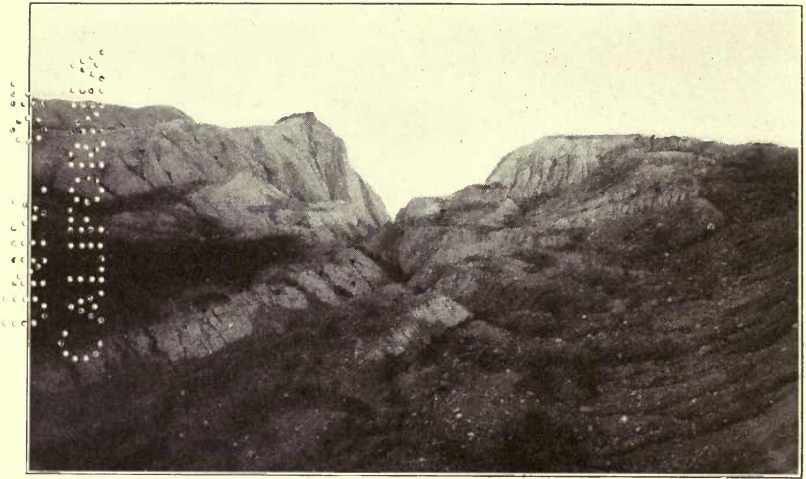
Fig. A. Abandoned clay pit near Fort Sheridan. [Courtesy of the C. & N. W. Ry.]
