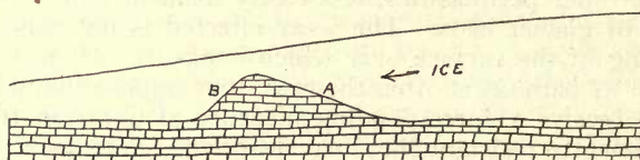
FIG. 5. The same hill after it has been eroded by the ice. A, the stoss side; B, the lee side.
