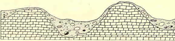
FIG. 9. Diagrammatic section showing relation of drift to underlying rock where the drift is thin relative to the relief of the underlying rock.
