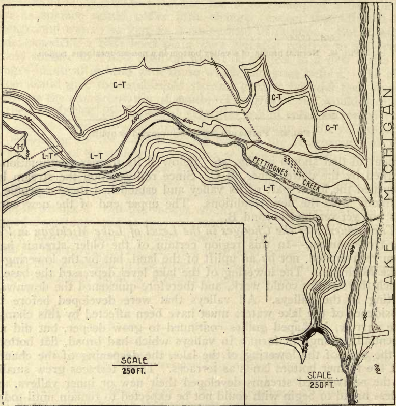
FIG. 48. Topographic map of the lower portion of Pettibone Creek valley near North Chicago, by Fred Kay and F. D. Mabrey. A broad terrace (C-T) corresponding to the Calumet stage of Lake Chicago is shown on the North side of the valley. In the bottom of the valley small remnants (T-T) correspond to the upper Toleston, and (L-T) to the lower Toleston stages of Lake Chicago.
