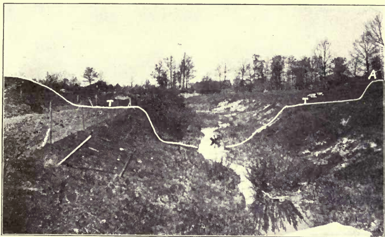
Fig. A. Little Fort creek in the western portion of Waukegan. These terraces probably espond to the Calumet stage of Lake Chicago as shown in the valley development.
