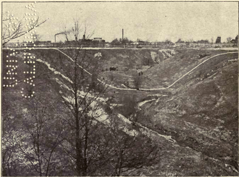
Fig. A. North fork of Pettibone creek, North Chicago.
