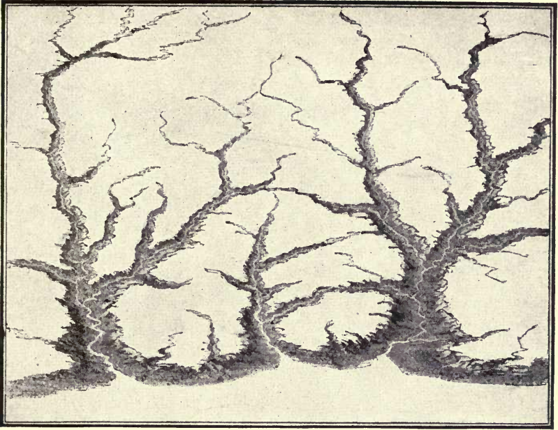
Fig. A. The same valleys as shown in plate 8, fig. B, in a later stage of development. [Courtesy of Wisconsin Geol. Nat. Hist. Surv.]
