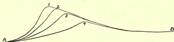
FIG. 38. Diagram showing the shifting of a divide. The slopes 1A and 1B are unequal. The steeper slope is worn more rapidly and the divide is shifted from 1 to 4, where the two slopes become equal and the migrating of the divide ceases.
