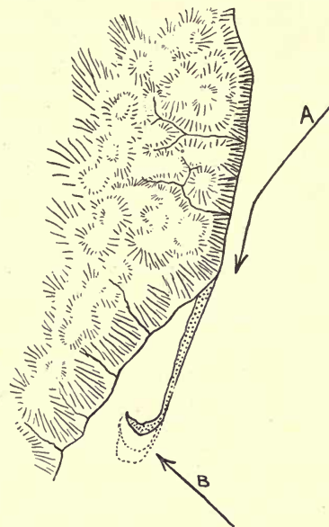
FIG. 26. Sketch map showing the development of a hooked spit.
