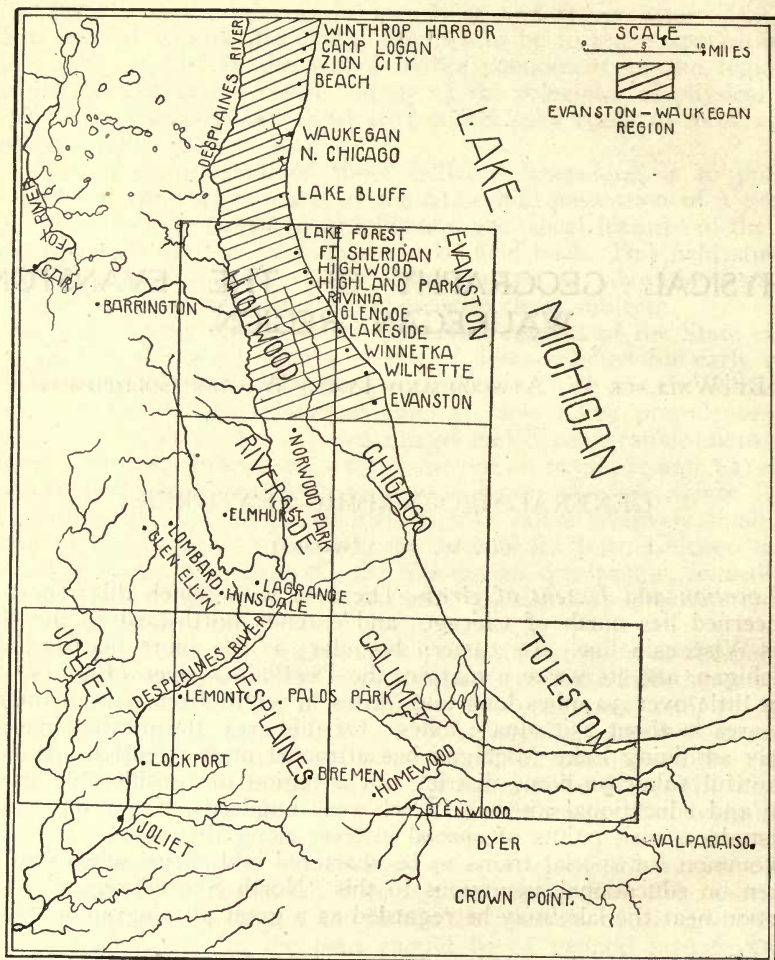
FIG. 1. General map showing location and extent of the Evanston-Waukegan region, the quadrangles for which topographic maps are available, and the chief points mentioned in the report.
