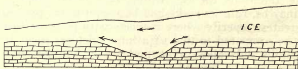
FIG. 6. Diagram showing effect on a valley of ice moving transversely across it.
