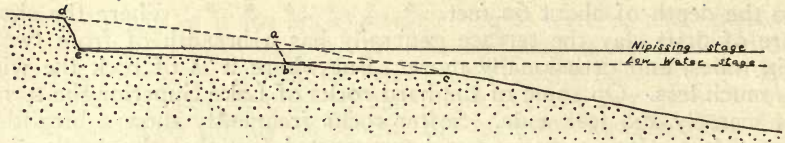
FIG. 29. Diagram showing how a deeply submerged terrace may have been developed by cliff recession during a rising of the water level from the low water stage to the "Nipissing" stage. (a b c) cliff and terrace cut during low water stage; (d e c) cliff and terrace after the rise and encroachment of waters.
