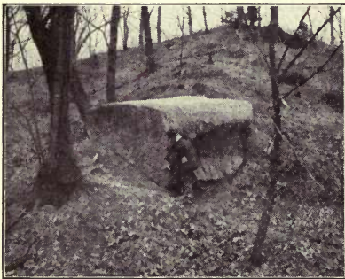
Fig. B. Limestone boulder in north fork of Pettibone Creek, North Chicago.
