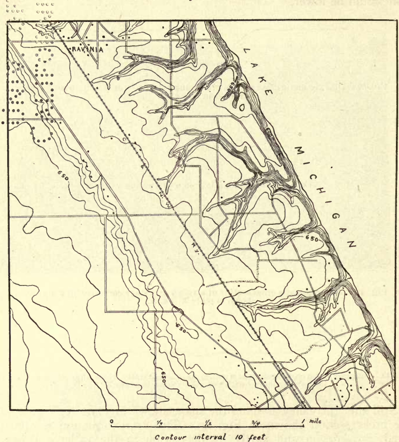
FIG. 44. Topographic map of a part of the North Shore near Ravinia, showing several young valleys.
