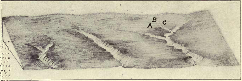
Fig. A. Moraine upland descending to lake shore.
