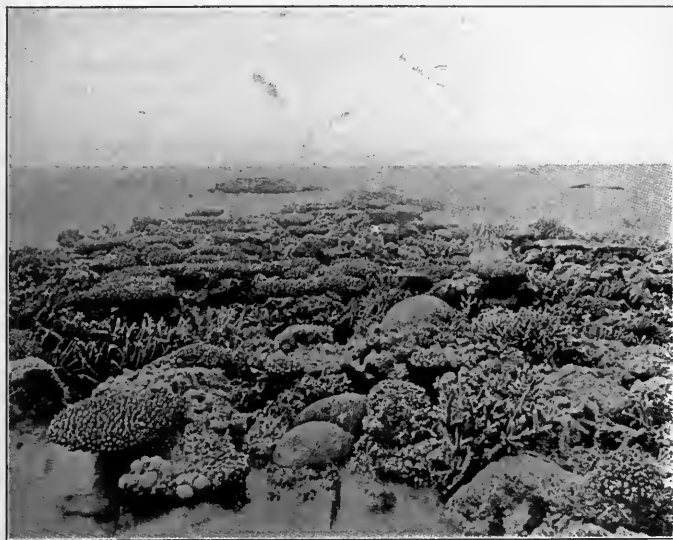
FIG. 509.—Coral growing.
