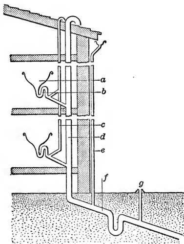
Diagram of the plumbing of a house.
