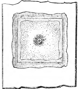
FIG. 43. In the centre is an assimilating alga.
