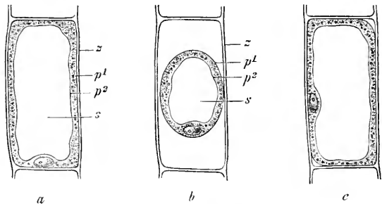
FIG. 4. Cells from the radicle of Zea Mays ( \times 375 ), (a) in water; (b) after plasmolysis in 5 per cent. \text{KNO}_3 ; (c) in 2.3 per cent. \text{KNO}_3 .
