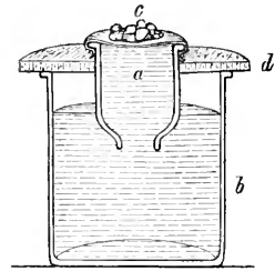
FIG. 18. The glass cylinder a is covered with parchment ( c ) and is filled with dilute hydrochloric acid, as is also the outer vessel ( b ). If pieces of marble are placed on c , in an hour or so the presence of calcium in the outer fluid may be demonstrated by the addition of oxalic acid and ammonia. (Optical section, one-fifth natural size.)
