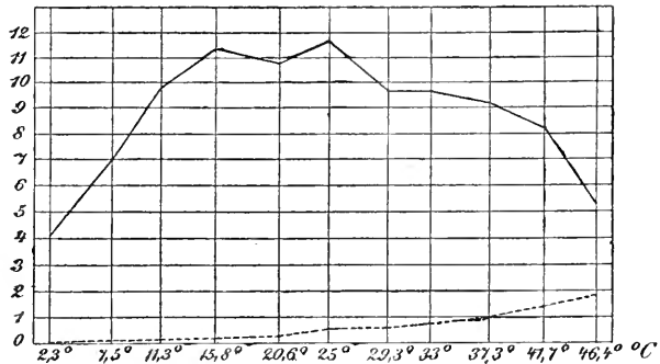
FIG. 50. Assimilation and respiration in a leafy branch of Rubus fruticosus at different temperatures (after Kreuzler). When assimilating, the branch is surrounded by air containing 0.3 per cent. CO 2 , and is illuminated by electric light (=bright diffuse daylight). By adding the height of the respiratory curve to that of the assimilatory one the actual amount of CO 2 assimilated is obtained. — CO 2 assimilated } per hour per sq. metre of leaf-surface. - - - - - CO 2 produced by respiration
