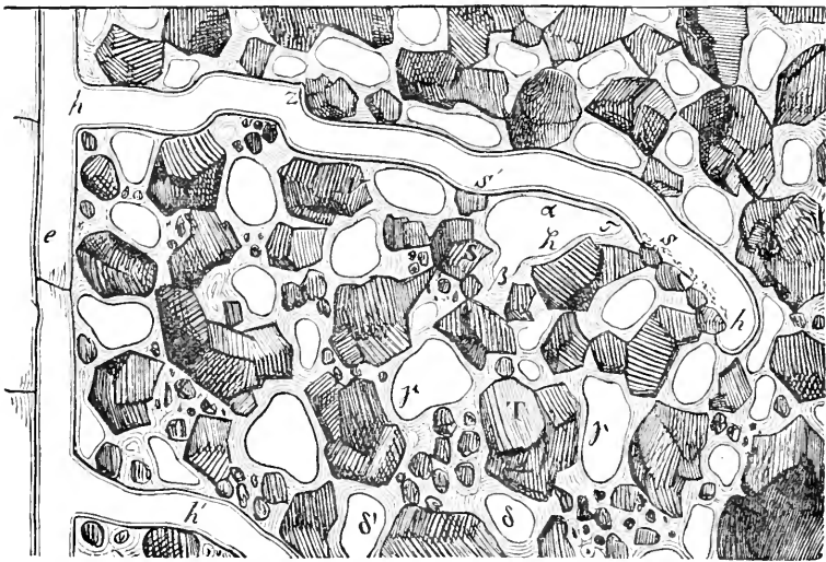
FIG. 16. From the root-epidermis (piliferous layer) the root-hairs h and h' arise. The solid soil particles are darkly shaded ( T ), the air spaces ( \beta , \gamma , &c.) are white, the adherent water is indicated by concentric lines. (After Sachs.)
