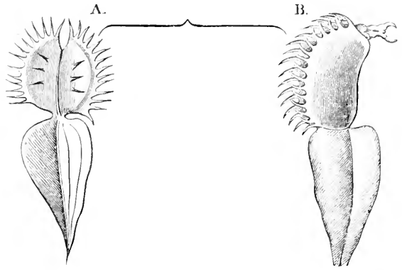
FIG. 57. Leaves of Dionaea muscipula . (A) opened, on each leaf-segment the three irritant hairs may be seen. (B) an earwig is captured between the closed leaf-segments.
