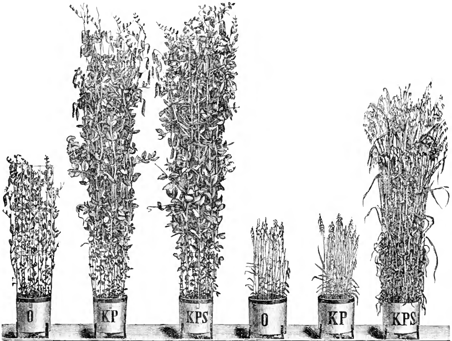
FIG. 60. The plants are grown (O) in soil containing hardly any combined nitrogen, to which (KP) potassium phosphate and (KPS) potassium phosphate and nitrate are added. The other ash constituents are already present, and also traces of combined nitrogen, so that feeble development is possible in (O). (After Wagner, Die rationelle Düngung , 1891, 2. Aufl., p. 13.)
