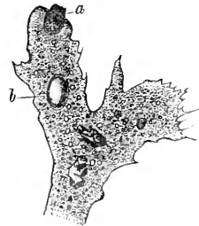
FIG. 7. Portion of a plasmodium of Chondrioderma difforme . A foreign body is being ingested at a , while internally various ingested particles are present, including an oil-drop, b . ( \times 200 )
