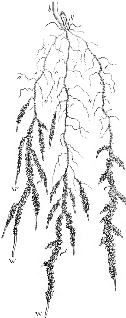
FIG. 13. Seedlings of Triticum vulgare grown in garden humus. After shaking, the earth adheres only to the portions bearing root-hairs, e' . At e no root-hairs are present and the lateral roots have in part died away. (After Sachs.)
