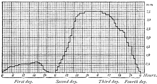
FIG. 4. Curve of grand period of growth of sporangiophore of Phycomyces nitens during development under favourable and constant external conditions. The ordinates give the hourly increments of growth in millimetres.
