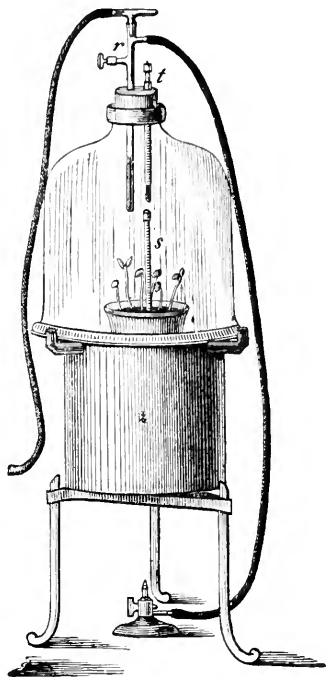
FIG. 17. Apparatus for constant temperature. Between the double walls of the zinc vessel z is water kept at constant temperature by the regulator r t and s are thermometers.
