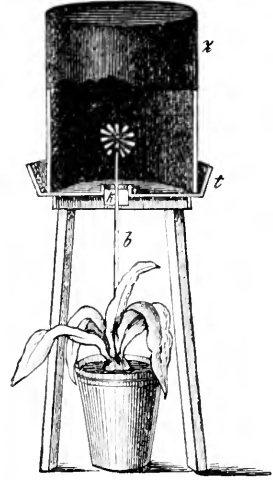
FIG. 23. Apparatus for partial etiolation. The apex of the flowering shoot a is passed through the opening k in the clay saucer l , which is closed by cork and cotton-wool. The dark cylinder z is pressed into the sand covering the floor of l .
