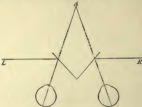
FIG. 87.—Wheatstone's stereoscope.
