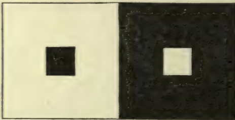
FIG. 69.—Irradiation.
