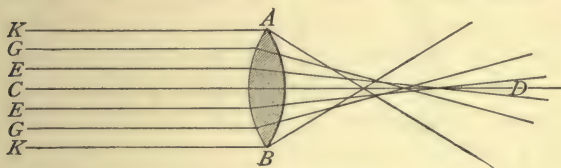
FIG. 55.—Spherical aberration.
