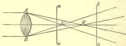
FIG. 56.—Chromatic aberration.
