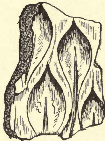
FIG. 13.— Lepidodendron aculeatum in sandstone.
