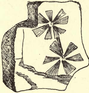
FIG. 10.— Sphenophyllum cuneifolium . Coal-shale.
