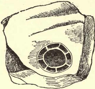
FIG. 17.—Section of stigmaria .
