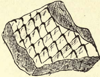
FIG. 12.— Lepidodendron longifolium . Coal-shale.
