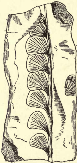
FIG. 3.— Rhacopteris inaequilatera . Carboniferous limestone.
