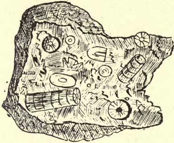
FIG. 21.—Encrinital limestone.
