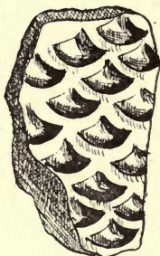
FIG. 30.— Lepidodendron . Portion of Sandstone stem after removal of bark of a giant club-moss.
