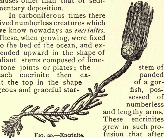
FIG. 20.—Encrinite.
