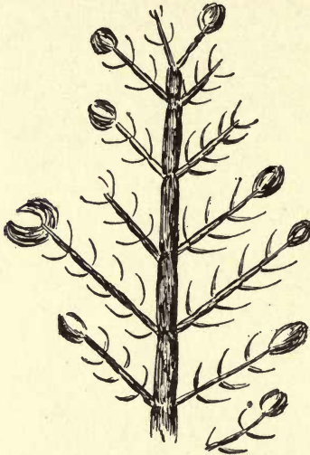
FIG. 8.— Calamocladus grandis . Carboniferous sandstone.
