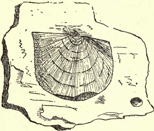
FIG. 29.— Aviculopecten papyraceus . Coal-shale.
