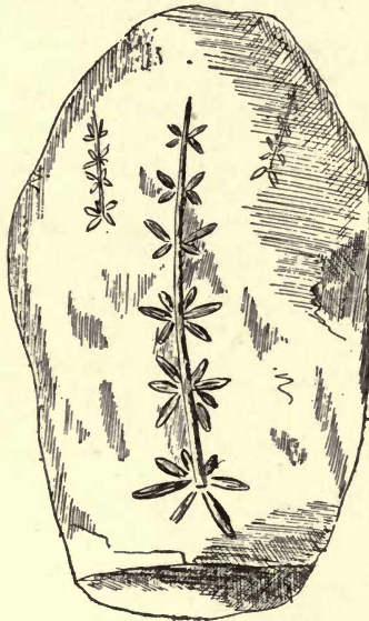
FIG. 2.— Annularia radiata . Carboniferous sandstone.
