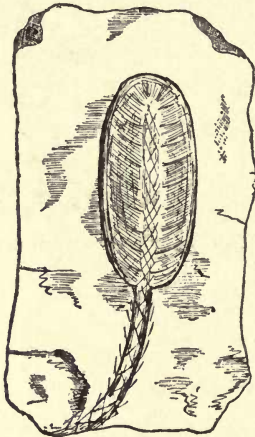
FIG. 14.— Lepidostrobus . Coal-shale.
