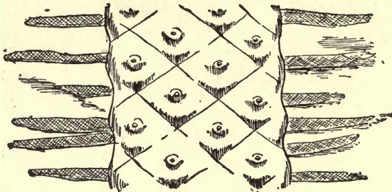
FIG. 16.— Stigmaria ficoides . Coal-shale.
