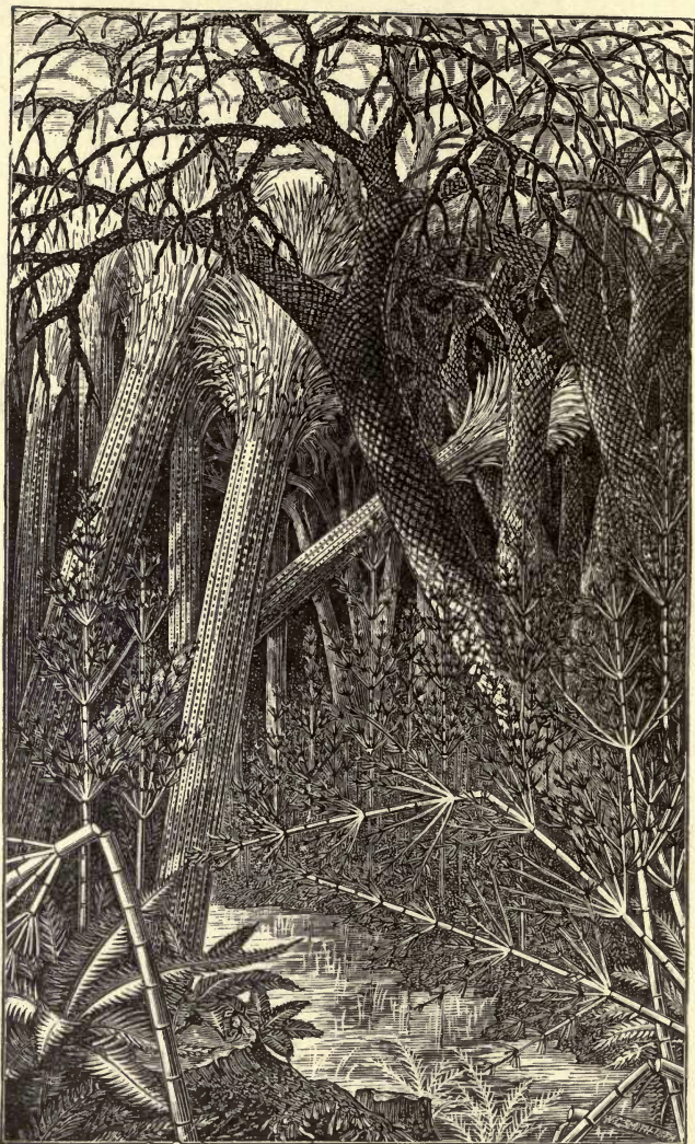
FIG. 1.—A Forest of the Coal period.
