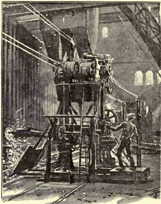
FIG. 35.—Filling Retorts by Machinery.
