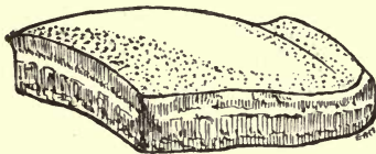
FIG. 25.— Psammodus porosus . Crushing palate of a fish.
