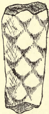
FIG. II.—Cast of Lepidodendron in sandstone.
