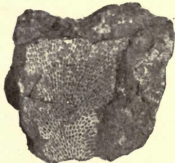
FIG. 27.— Fenestella retipora . Mountain limestone.
