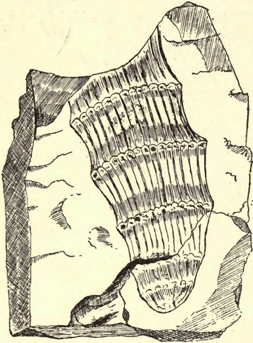
FIG. 7.—Root of Calamites Suckowii . Coal-shale.
