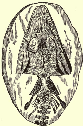
FIG. 24.— Archegosaurus minor . Coal-measures.
