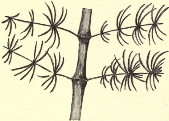
FIG. 9.— Asterophyllites foliosa . Coal-measures.
