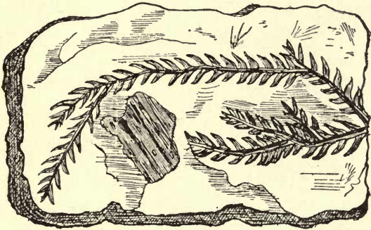
FIG. 15.— Lycopodites . Coal sandstone.
