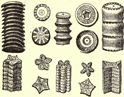
FIG. 22.—Encrinites : various. Mountain limestone.
