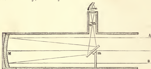
FIG. 82.—Principle of Newtonian reflector.
