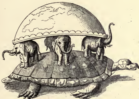
FIG. 6.—Hindoo Earth.
