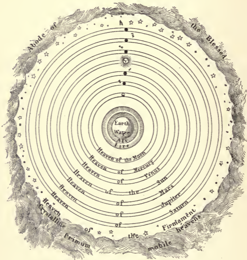
FIG. 8.—Ptolemaic system.
