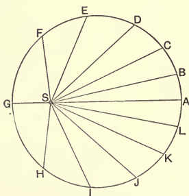
FIG. 30.—Excentric circle supposed to be divided into equal areas. The sun, S , being placed at a selected point, it was possible to represent the varying speed of a planet by saying that it moved from A to B , from B to C , and so on, in equal times.
