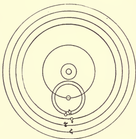
FIG. 11.—Egyptian system.
