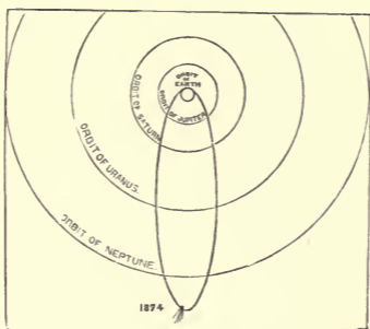
FIG. 99.—Orbit of Halley's comet.
