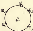
FIG. 12.—True orbits of Earth and Jupiter.
