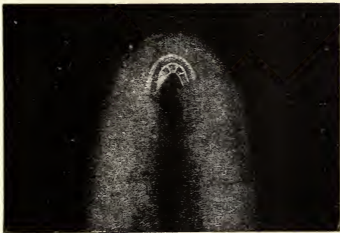
FIG. 88.—Old drawing of the Andromeda nebula.
