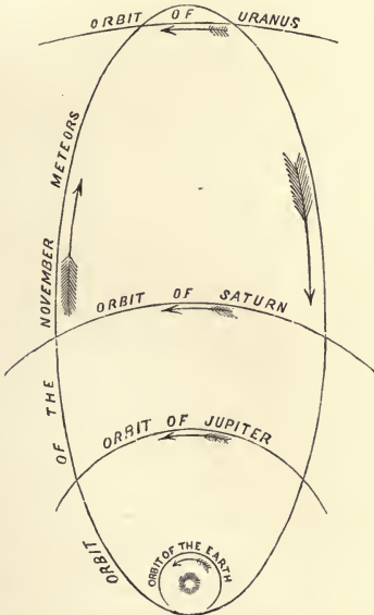
FIG. 106.—Orbit of November meteors.
