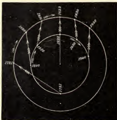
FIG. 94.—Uranus's and Neptune's relative positions.
