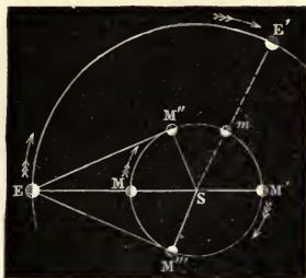
FIG. 13.—Orbit of Mercury and Earth.
