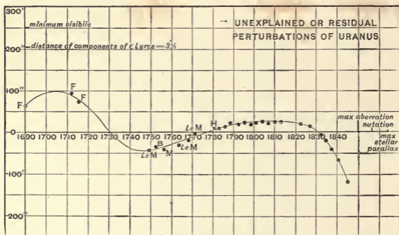
FIG. 93.—Perturbations of Uranus.
