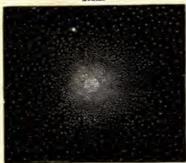
FIG. 43.—Some clusters and nebulae.
