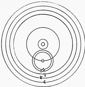
FIG. 11.—Egyptian system.
