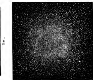
FIG. 43.—Some clusters and nebulae.
