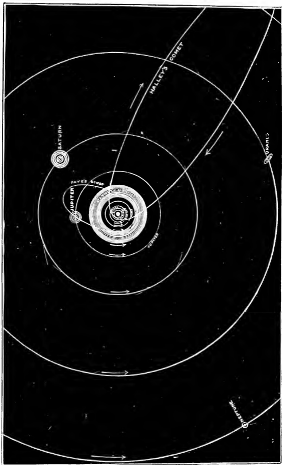
FIG. 90.—Planetary orbits, etc.; showing the Asteroidal belt between the planets of Mars. (The orbits of satellites are exaggerated.)
