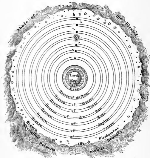
FIG. 8.—Ptolemaic system.
