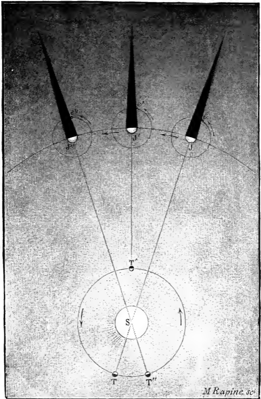
FIG. 75.—Eclipses of one of Jupiter's satellites. A diagram intended to illustrate the dependence of its apparent time of revolution (from eclipse to eclipse) on the motion of the earth; but not illustrating the matter at all well. TT' T'' are successive positions of the earth, while JJ' J'' are corresponding positions of Jupiter.
