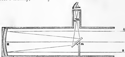
FIG. 82.—Principle of Newtonian reflector.
