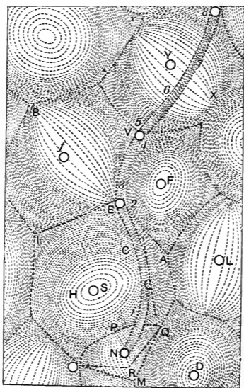
FIG. 55.—Descartes's diagram of vortices, from his Principia .
