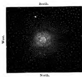
FIG. 43.—Some clusters and nebulae.
