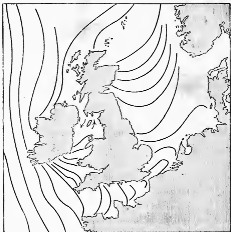
FIG. 109.—Co-tidal lines.
