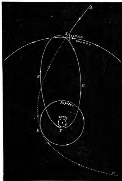
FIG. 167.—Orbit of November meteors; showing their probable parabolic orbit previous to 126 A.D., and its sudden conversion into an elliptic orbit by the violent perturbation caused by Uranus, which at that date occupied the position shown.
