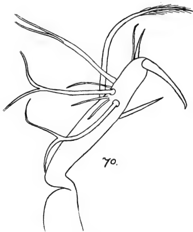
Fig. 70. Th. bernardensis . Terminal portion of left antenna; only the primary bifurcation of the branched setae is shown.
