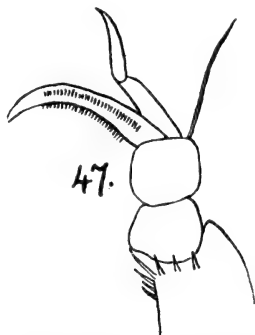
Fig. 47. H. uniremis ♂. Terminal portion of p 1 Ri; from station 13.
