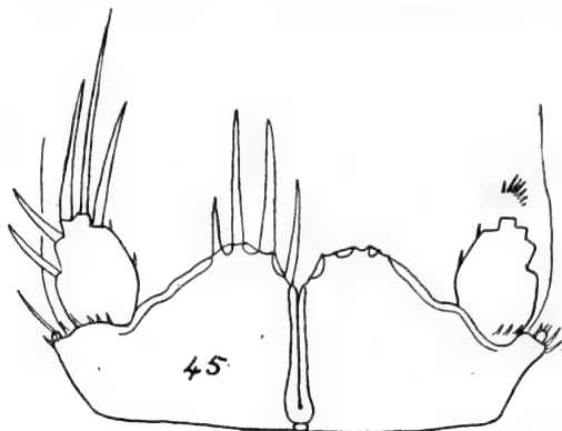
Fig. 45. Harpacticus superflexus . Fifth legs of female.
