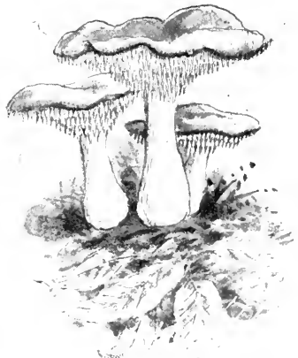
FIG. 65. Hydnum repandum , in which gills are replaced by spinous processes; edible.—After GIBSON.
