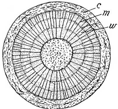
FIG. 79. Section across a twig of box elder three years old, showing three annual rings, or growth rings, in the vascular cylinder. The radiating lines ( m ) which cross the vascular region ( w ) represent the pith rays, the principal ones extending from the pith to the cortex ( c ).
