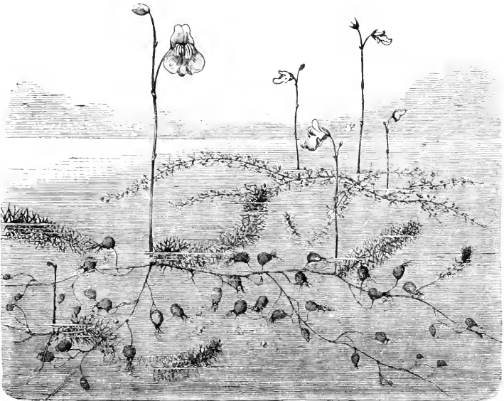
FIG. 155. Bladderwort, showing the numerous bladders which float the plant, the finely divided water leaves, and the erect flowering stems. The bladders are also effective "insect traps," Utricularia being one of the "carnivorous plants." —After KERNER.
