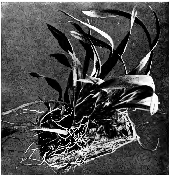
FIG. 93. An orchid, showing aerial roots.
