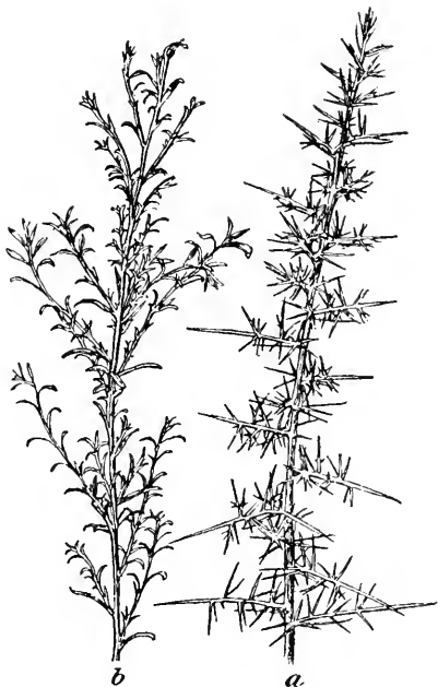
FIG. 177. Two plants of common gorse or furze ( Ulex ), showing the effect of environment: b is a plant grown in moist conditions; a is a plant grown in dry conditions, the leaves and branches having been almost entirely developed as thorns.—After LOTHÉLIER.
