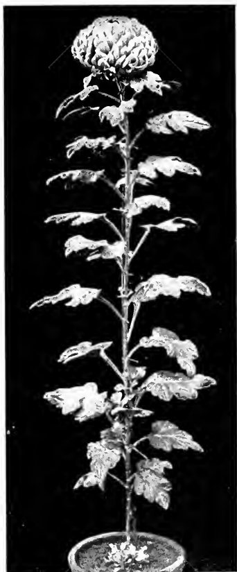
FIG. 17. A chrysanthemum, showing lobed leaves, the rising of the petioles to adjust the blades to light, and the general cylindrical habit.
