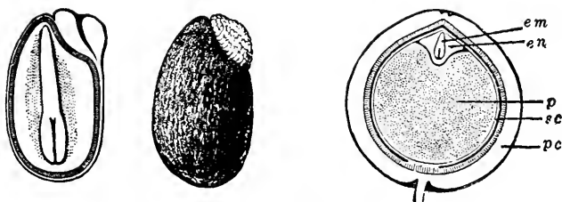
FIG. 183. The two figures to the left are seeds of violet, one showing the black, hard testa, the other being sectioned and showing testa, endosperm, and imbedded embryo; the figure to the right is a section of a pepper fruit ( Piper ), showing modified ovary wall ( pc ), seed testa ( sc ), nucellus tissue ( p ), endosperm ( en ), and embryo ( em ).—After BAILLON.
