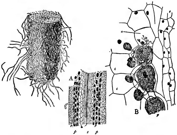
FIG. 76. Mycorrhiza: to the left is the tip of a rootlet of beech enmeshed by the fungus; A, diagram of longitudinal section of an orchid root, showing the cells of the cortex ( p ) filled with hyphae; B, part of longitudinal section of orchid root much enlarged, showing epidermis ( e ), outermost cells of the cortex ( p ) filled with hyphal threads, which are sending branches into the adjacent cortical cells ( a , i ).—After FRANK.
