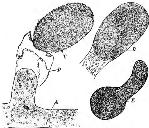
FIG. 9. Vaucheria geminata , a Siphon form, showing a portion of the cenocytic body (A) which has sent out a branch at the tip of which a sporangium (B) formed, within which a large zoospore was organized, and from which (D) it is discharged later as a large multiciliate body (C), which then begins the development of a new cenocytic body (E).—CALDWELL.
