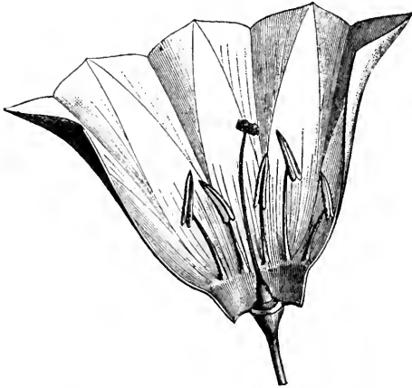
FIG. 209. Flower of morning-glory ( Ipomœa ), with sympetalous corolla split open, showing the five attached stamens, and the superior ovary with prominent style and stigma; the flower is hypogynous, sympetalous, and actinomorphic.—After MEISSNER.
