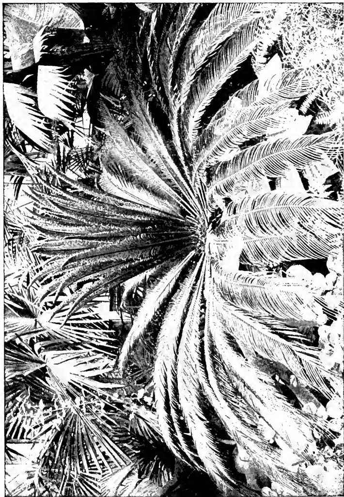
FIG. 156. Cycas revoluta , showing the foliage at the summit of the stem. In the center is the nearly erect cluster of young foliage leaves, below are the scale leaves which covered them in bud, and below these are the widely spreading old foliage leaves. —CALDWELL.
