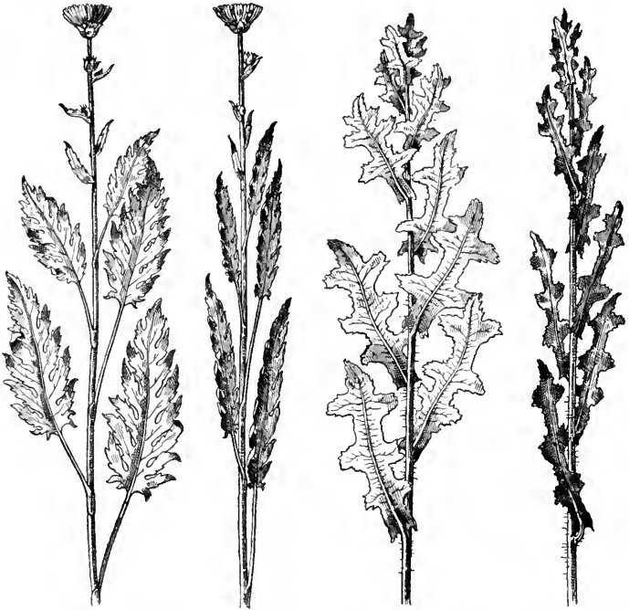
FIG. 170. Two compass plants. The two figures to the left represent the same plant ( Silphium ) viewed from the east and from the south. The two figures to the right represent the same relative positions of the leaves of Lactuca .—After KERNER.
