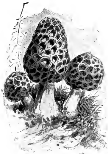
FIG. 47. The common edible morel ( Morchella esculenta ). The structure shown and used represents the ascocarp, the depressions of whose surface are lined with asci containing ascospores.—After GIBSON.
