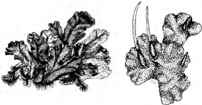
FIG. 93. Two common liverworts: to the left is Conocephalus , a Marchantia form, showing rhizoids, dichotomous branching, and the conspicuous rhombic areas (areolæ) on the dorsal surface; to the right is Anthoceros , with its simple thallus and pod-like sporogonia.—GOLDBERGER.
