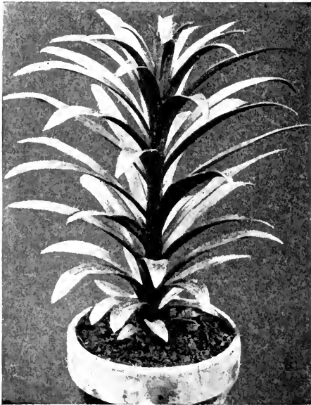
FIG. 7. An Easter lily, showing narrow leaves and numerous vertical rows.
