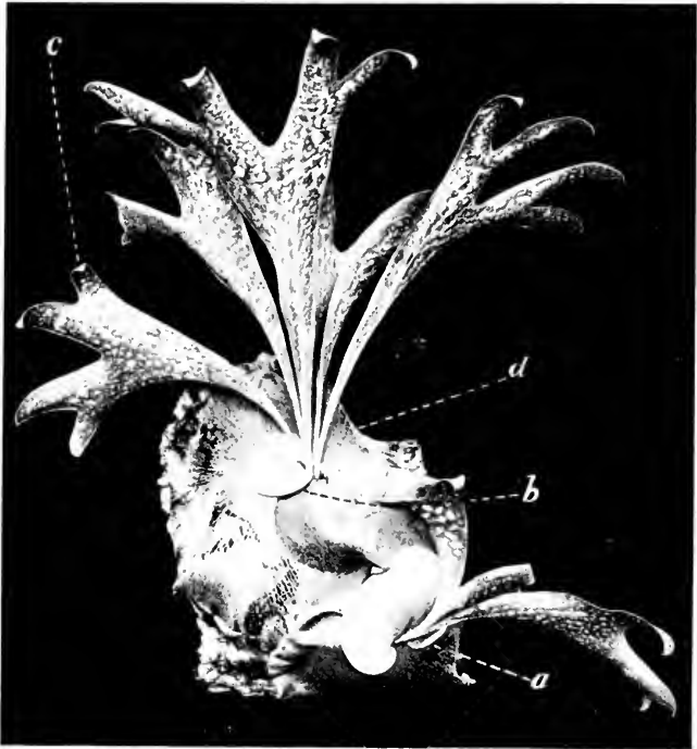
FIG. 112. Stag-horn fern ( Platycerium grande ), an epiphytic tropical form, showing the two forms of leaves: a and b , young sterile leaves; c , leaves bearing sporangia; d , an old sterile leaf.—CALDWELL.
