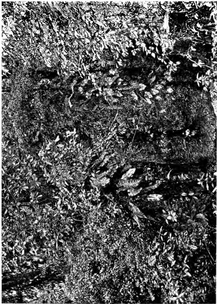
FIG. 242. A rainy tropical forest. Note the density of the vegetation, the abundance of lianas (climbers), and the general branching (compound) character of the leaves.—After SCHUMPER.
