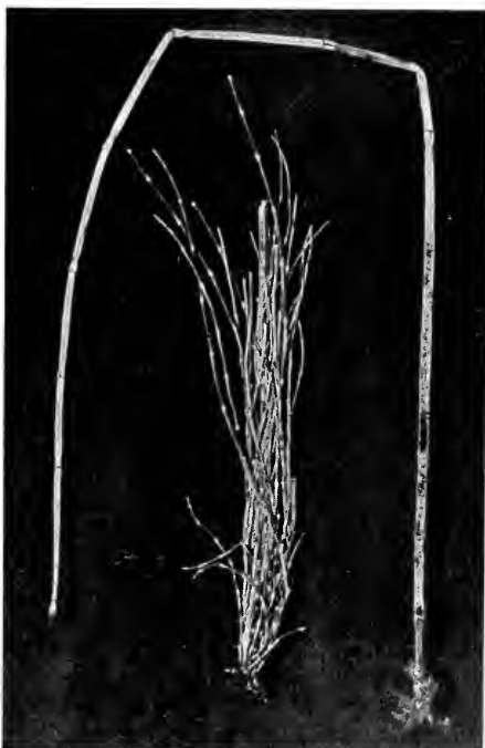
FIG. 175. Two plants of a common scouring rush ( Equisetum ), showing the effect of environment; the long, unbranched one having grown in normal mesophytic conditions; the short, bushy branching, more slender form having grown on the dunes (xerophyte conditions).—After COWLES.
