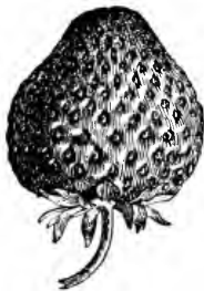
FIG. 191. Fruit of strawberry, showing the persistent calyx, and the enlarged pulpy receptacle in which numerous simple and dry fruits (akenes) are imbedded.—After BAILEY.
