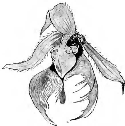
FIG. 142. A bee escaping from the pouch of Cyrtopodium , and rubbing against an anther.—After GIBSON.
