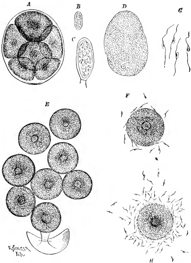
FIG. 21. Sexual reproduction of Fucus , showing the eight eggs (six in sight) discharged from the oogonium and surrounded by a membrane (A), eggs liberated from the membrane (E), antheridium containing sperms (C), the discharged laterally biciliate sperms (G), and eggs surrounded by swarming sperms (F, H).—After SINGER.
