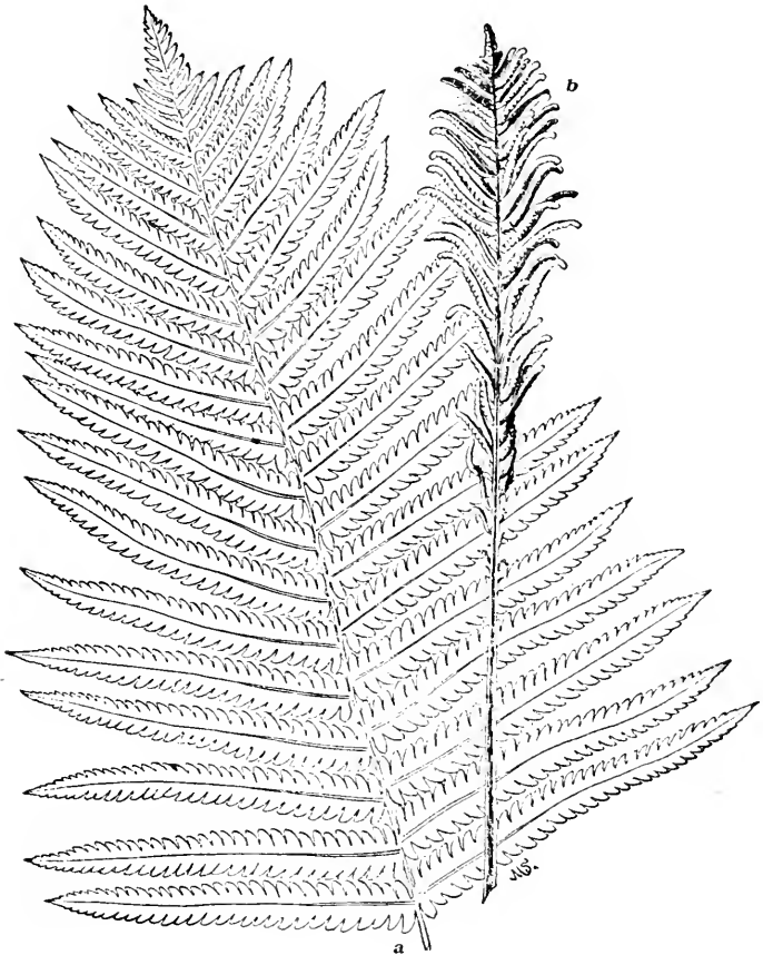
FIG. 137. The ostrich fern ( Onoclea struthiopteris ), showing differentiation of foliage leaf (a) and sporophyll (b).—After MARION SATTERLEE.
