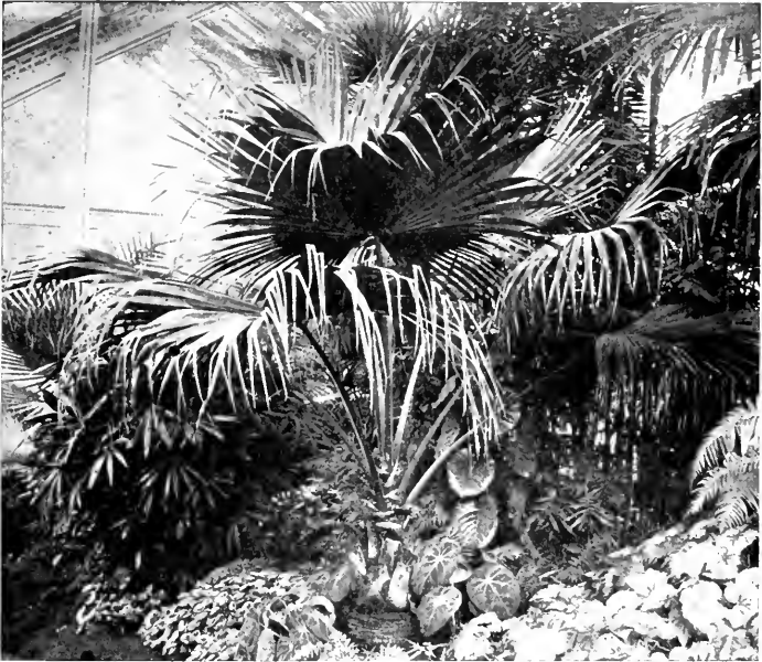
FIG. 82. A palm of the palmetto type (fan palm), with low stem and a crown of large leaves.
