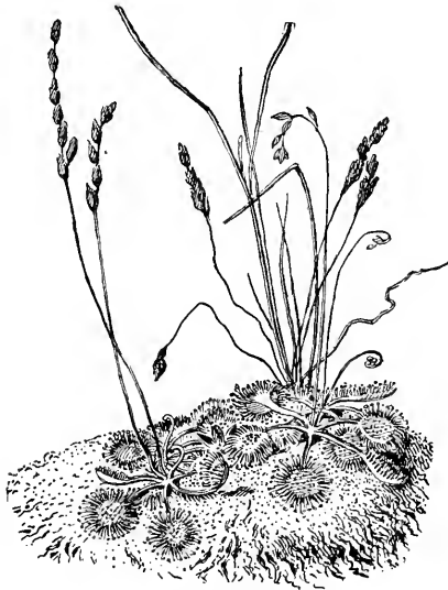
FIG. 149. A sun-dew, showing rosette habit of the insect-catching leaves.
