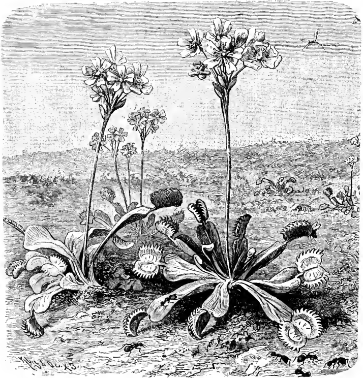
FIG. 151. Plants of Dionaea , showing the rosette habit of the leaves with terminal traps, and the erect flowering stem.—After KERNER.
