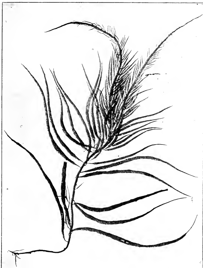
FIG. 25. A red alga ( Rabdonia ), showing holdfasts and branching thallus body.— CALDWELL.
