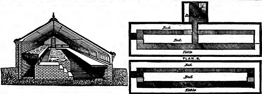
THREE-QUARTER SPAN GREENHOUSE FOR ROSE FORCING, ETC.
