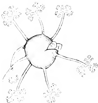
FIG. 42. Ascocarp of the lilac mildew, showing branching appendages and two asci protruding from the ruptured wall and containing ascospores. —S. M. COULTER.
