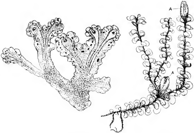
FIG. 99. Two liverworts, both Jungermannia forms; to the left is Blasia , which retains the thallos form but has lobed margins; to the right is Scapania , with distinct leaves and sporogonia (A).—GOLDBERGER.
