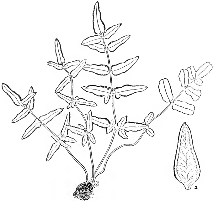
FIG. 136.—The purple cliff brake ( Pellea atropurpurea ), showing general habit, and at a a single leaflet showing the dichotomous venation and the infolded margin covering the sori.—After MARION SATTERLEE.
