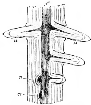
FIG. 277. Endogenous origin of root branches, showing them ( n ) arising from the central axis ( f ) and breaking through the cortex ( v ).—After VINES.
