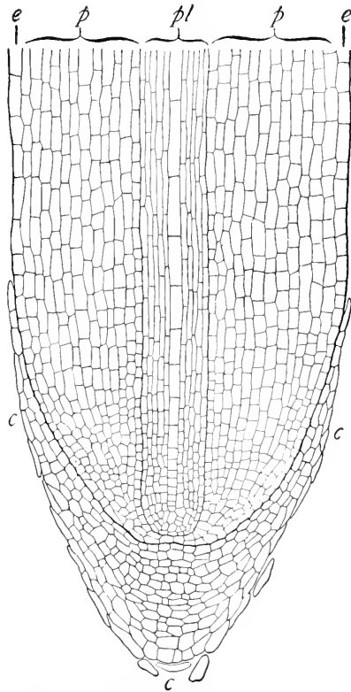
FIG. 275. A longitudinal section through the root-tip of spiderwort, showing the plerome ( pl ), surrounded by the periblem ( p ), outside of periblem the epidermis ( e ) which disappears in the older parts of the root, and the prominent root-cap ( c ).—LAND.
