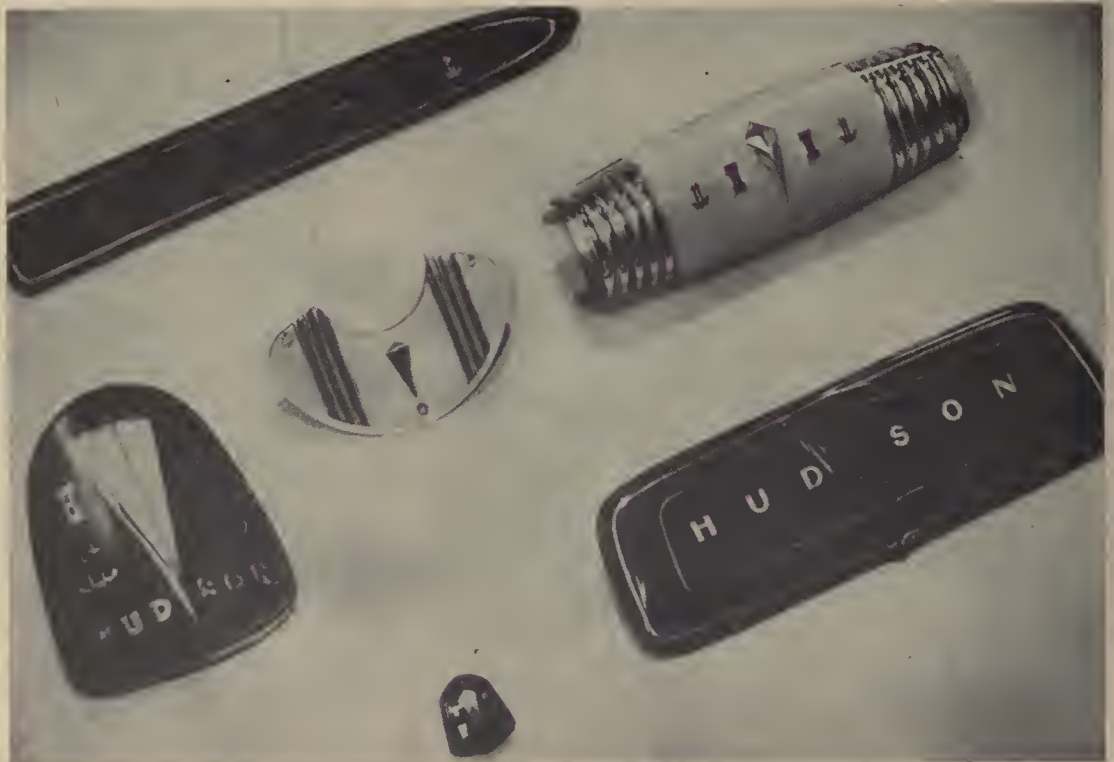
Hudson automobile parts molded of Plexiglas V, Rahm & Haas molding powder, by Gits Molding Corp., Chicago.
