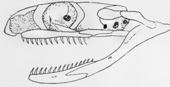
Fig. 4. PROFILE OF SKULL OF LAMPROPELTIS (After Jan.)
