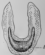
Fig. 2. CROSS-SECTION OF GROOVED FANG OF TRAGOPS PRASINUS, NEAR BASE. Enlarged. a Poison groove; b pulp cavity. (After Niemann.)
