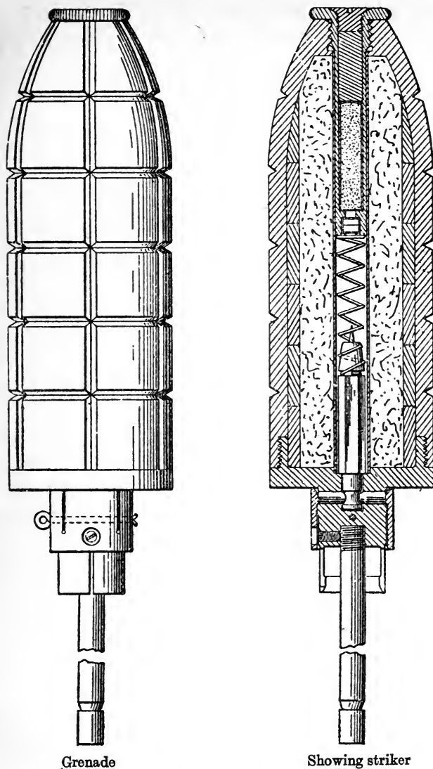
FIG. 5. Apparatus for throwing a grenade from a rifle, instead of by hand (Hale's patent).
