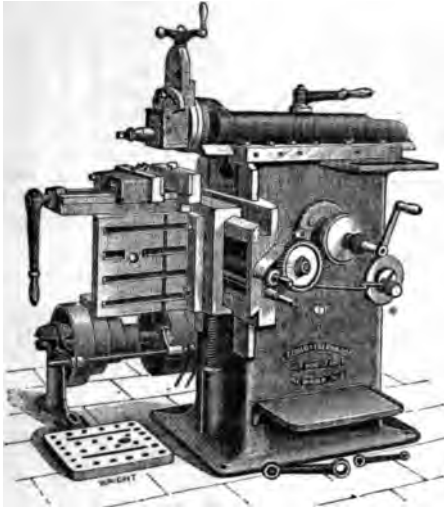
Patent SHAPERS. OVER 1000 IN USE. Sizes, 10' 15' 20' 25' 30'
