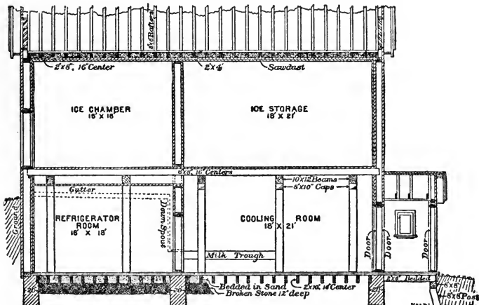
Fig. 72. —Kansas Cold Storage House; longitudinal section.
