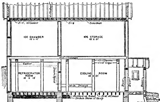
Fig. 72. —Kansas Cold Storage House; longitudinal section.
