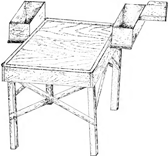
Fig. 70.—Sorting table for fruit packed in boxes.
