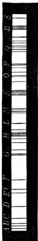
FIG. 2.—SOLAR SPECTRUM WITH THE ULTRA-VIOLET PORTION
