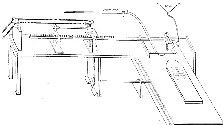
FIG. 8.—TILGHMAN'S SAND-BLAST STONE-MACHINE.
