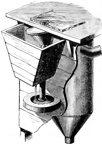
FIG. 6.—MACHINE OPERATED BY EXHAUST INSTEAD OF BLAST.
