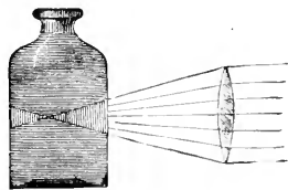
FIG. 1.—ILLUSTRATION OF FLUORESCENCE.
