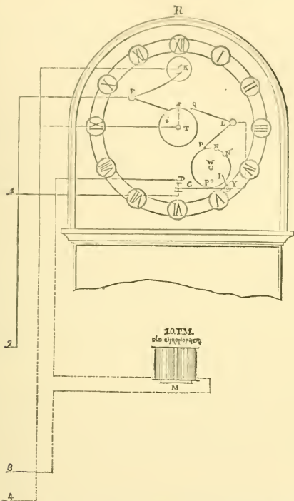
FIG. 9.—DIAGRAM SHOWING ELECTRIC CONNECTIONS OF CLOCK WITH CHRONOPHER.
