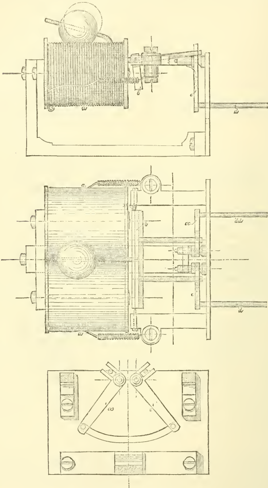
FIG. 12.—THE SYNCHRONIZER.
