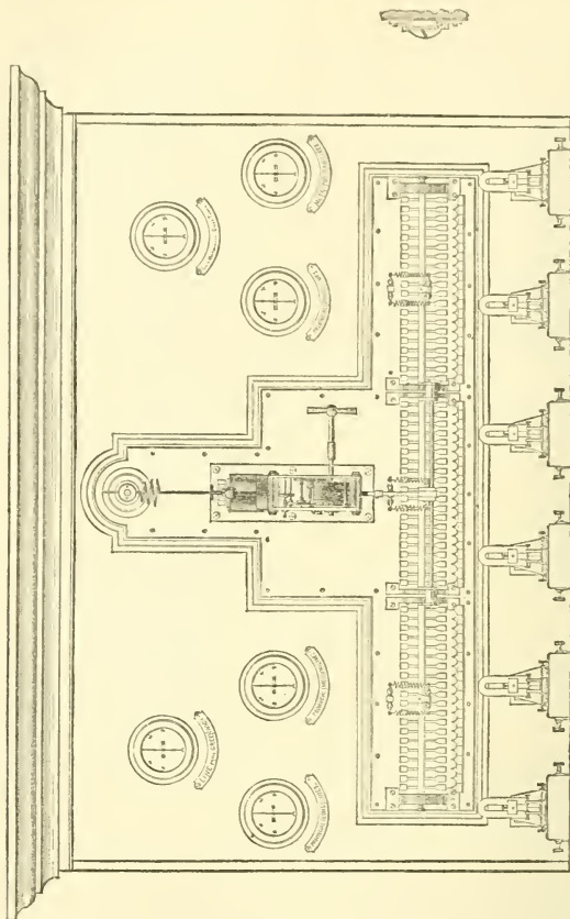
FIG. 7.—THE CHRONOPHER.—ELEVATION.
