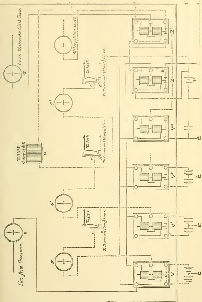
FIG. 8.—DIAGRAM SHOWING ELECTRIC CONNECTIONS OF THE CHRONOMETER.
