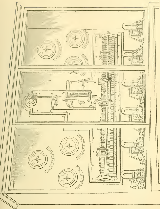
FIG. 6.—THE CHIRONOMIER.—PERSPECTIVE.
