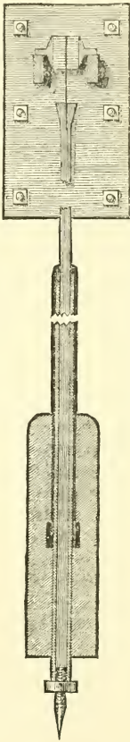
FIG. 3.—GREENWICH PENDULUM. SECTION.
