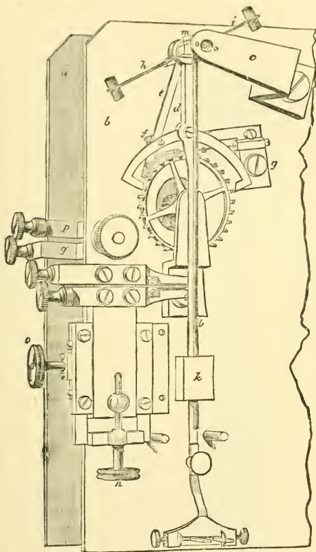
FIG. 1.—GREENWICH CLOCK ESCAPEMENT.
