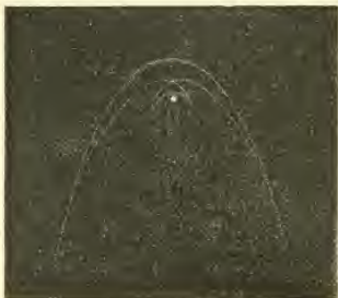
FIG. 2.—HEAD OF COMET SEPTEMBER 19— 5-INCH TELESCOPE.
