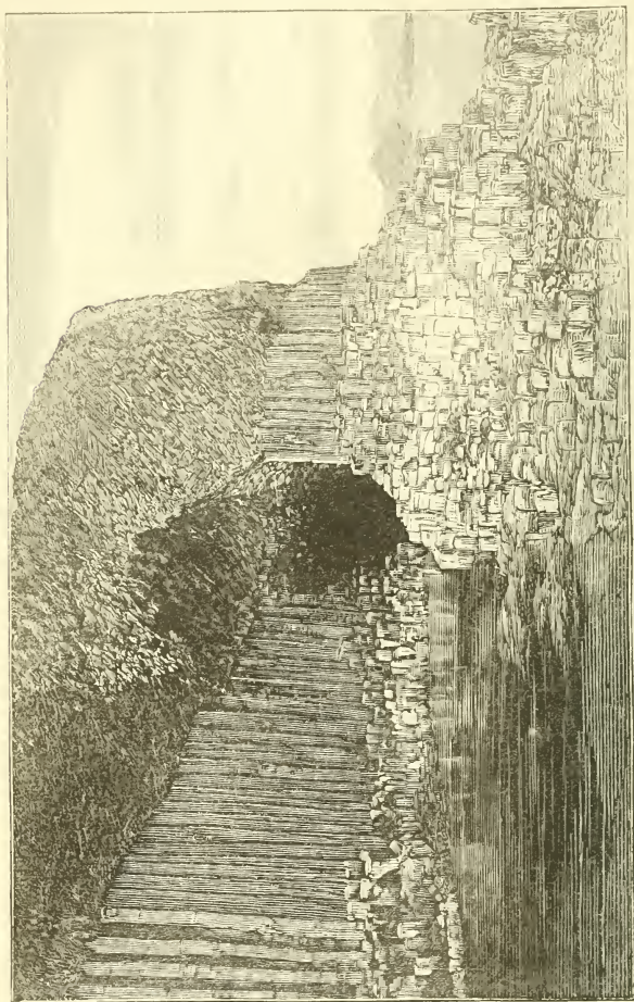
FIG. 3.—FINGAL'S CAVE, STAFFA, 1111. J. V.
