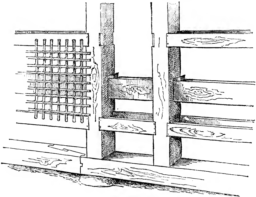
FIG. 1.—SIDE-FRAMING.
