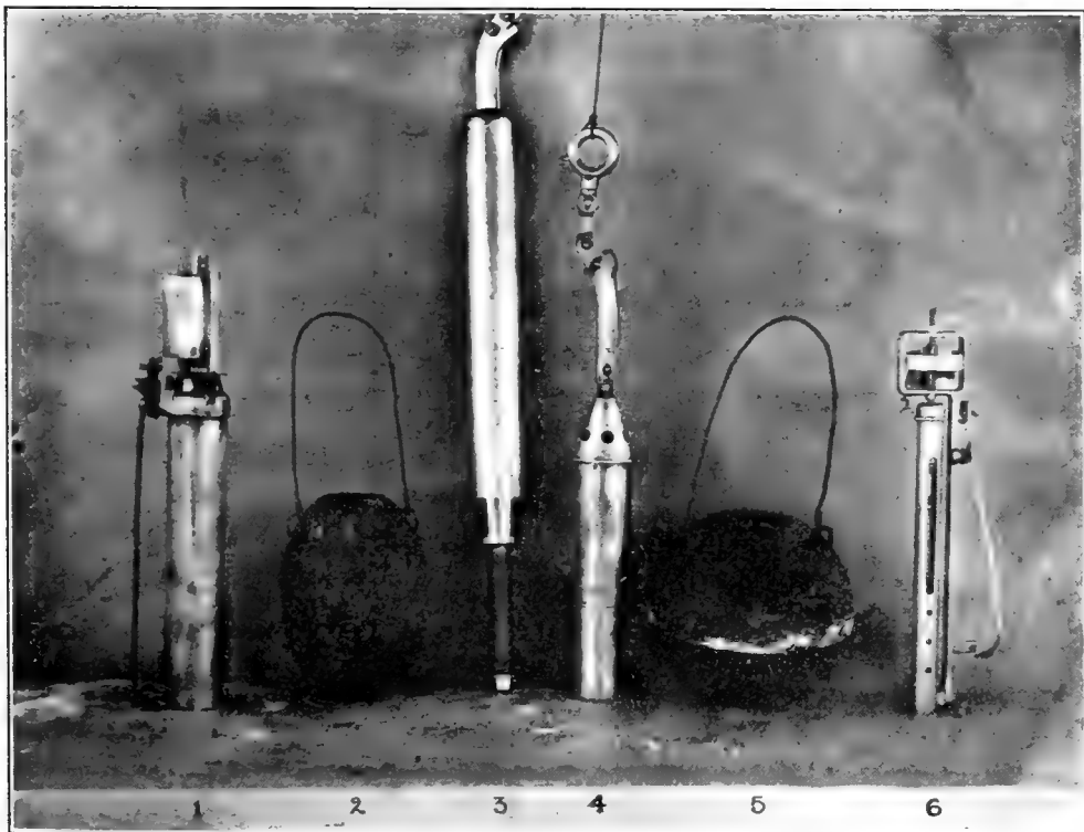
A SET OF SOUNDING INSTRUMENTS. 1, water bottle; 2, thirty-five-pound shot; 3, Thompson bail-cutting sounding rod; 4, bottom specimen cup; 5, sixty-pound shot; 6, deep-sea thermometer. (Photograph by DeLong.)
