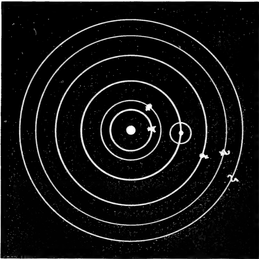
THE SOLAR SYSTEM AS CONCEIVED BY COPERNICUS.
