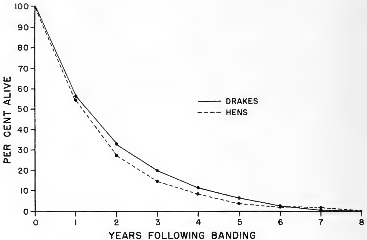
Fig. 3.--Survival rates of mallard drakes and mallard hens banded at Lake Chautauqua, 1939-1944.
