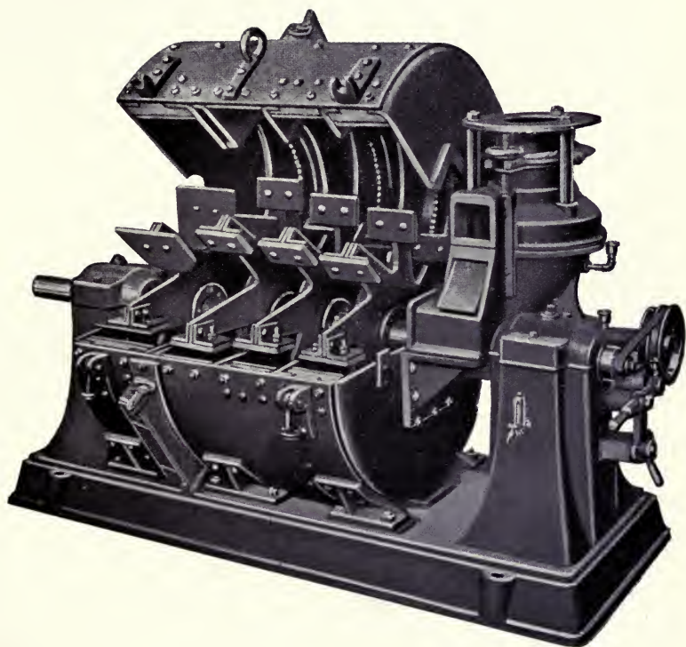
AERO PULVERIZER.
