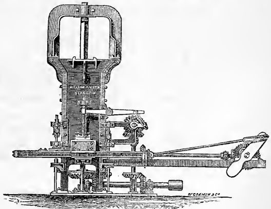
Improved Patent Brickmaking Machine.
