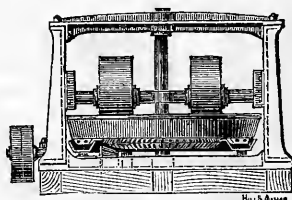
Improved Mortar Mill with Riddle Bottom.
