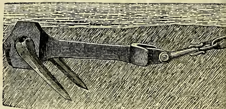
SIDE VIEW OF THE ANCHOR EMBEDDED INTO THE GROUND WHEN HOLDING
