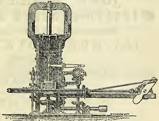
Improved Patent Brickmaking Machine.
