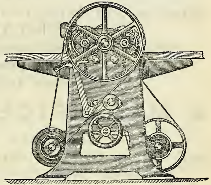
Improved Wood Planer.
