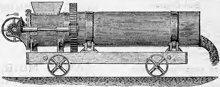
JAMIESON'S PATENT CONCRETE MACHINE.
