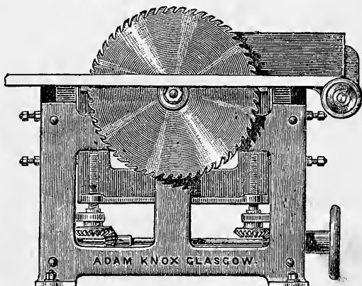
Illustration of Bench for 24 inch Saws, with Top 4 ft. by 2 ft. 2 in.
