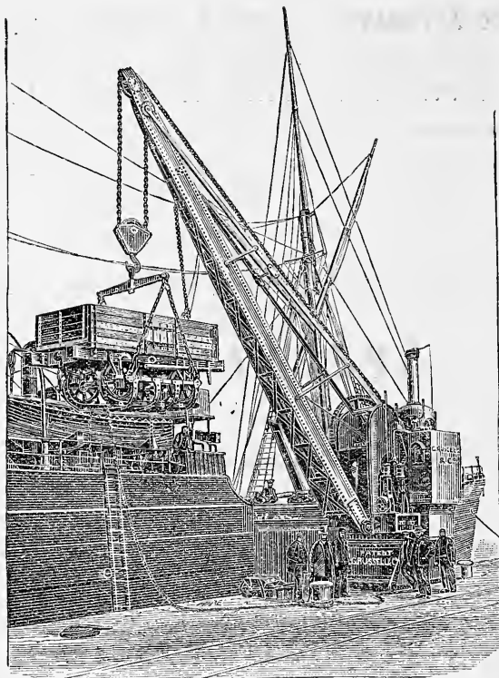
RUSSELL'S PATENT SEMI-PORTABLE 30 TONS COALING CRANES, AT GENERAL TERMINUS, GLASGOW HARBOUR.
