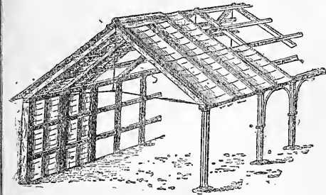
Shed, with Patent Steel unbreakable Pillars and Patent Arc Tube-jointing Sheets in Roof and Side.
