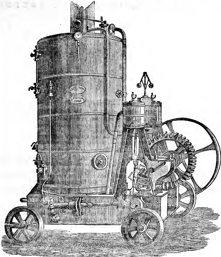
THE 'FIELD' BOILER, AND ENGINE ATTACHED.
