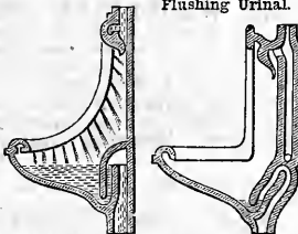
Flat Back (in use). (Cradle after Siphonage.)
