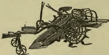
FIG. 44—THE HOOVER DIGGER
