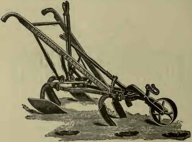
FIG. 31—FIVE-TOOTH CULTIVATOR WITH HILLER ATTACHMENTS Still used by many farmers.
