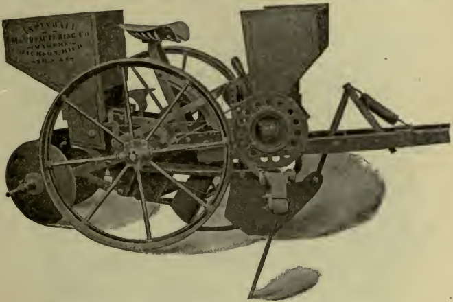
FIG. 27—ASPINWALL POTATO PLANTER (SIDE VIEW)
