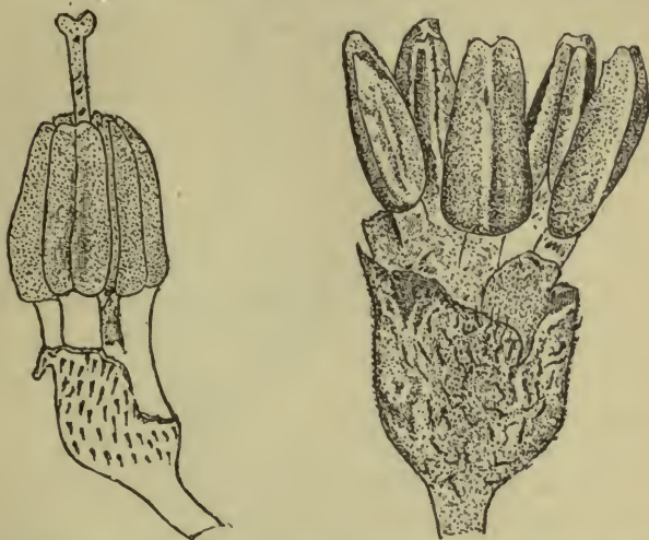
FIG. 50—POTATO FLOWER, WITH CALYX AND COROLLA REMOVED On the left are shown the anthers closed round the pistil. On the right the anthers are expanded, pistil not shown. The inner surfaces of the anthers show the line where rupture occurs when the pollen is liberated. Generally this occurs only near the upper portion of the anther.
