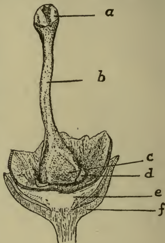
FIG. 51 — PISTIL OF POTATO FLOWER, SHOWING THE PARTS
