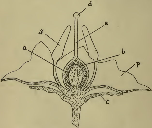
FIG. 3—SECTIONAL VIEW OF POTATO FLOWER ( Diagrammatic )
