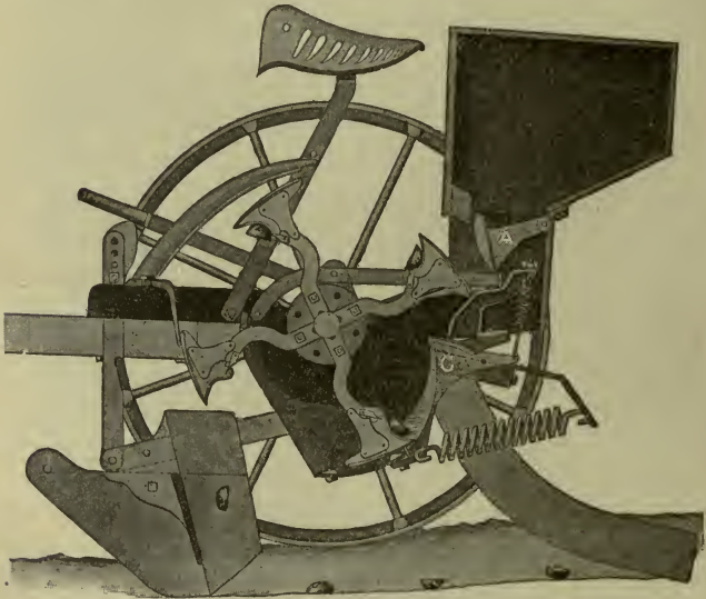
FIG. 26—SECTIONAL VIEW OF ASPINWALL PLANTER
