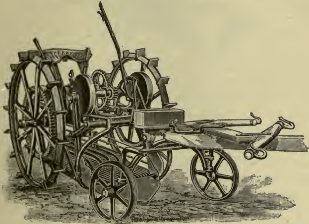
FIG. 43—THE REUTHER POTATO DIGGER
